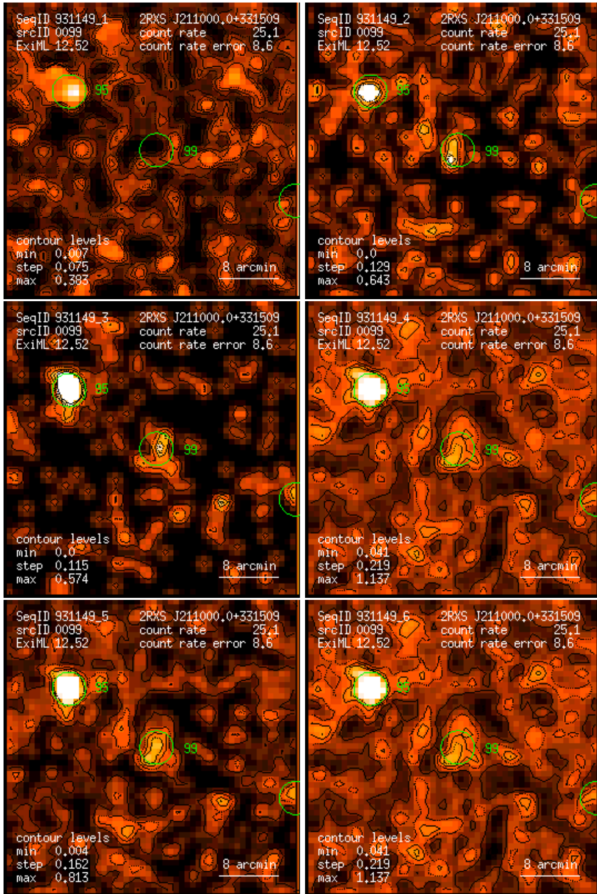
Figure 99: RASS 931149: detection 0099: band rate images, Gaussian filter: (1) PSPC channels 11 – 41, (2) 52 – 90, (3) 91 – 201, (4) 11 – 235, (5) 52 – 201, (6) 11 – 201. Broad band rates in counts/ks. Band rate contour levels in counts/ks/arcmin 2 .
