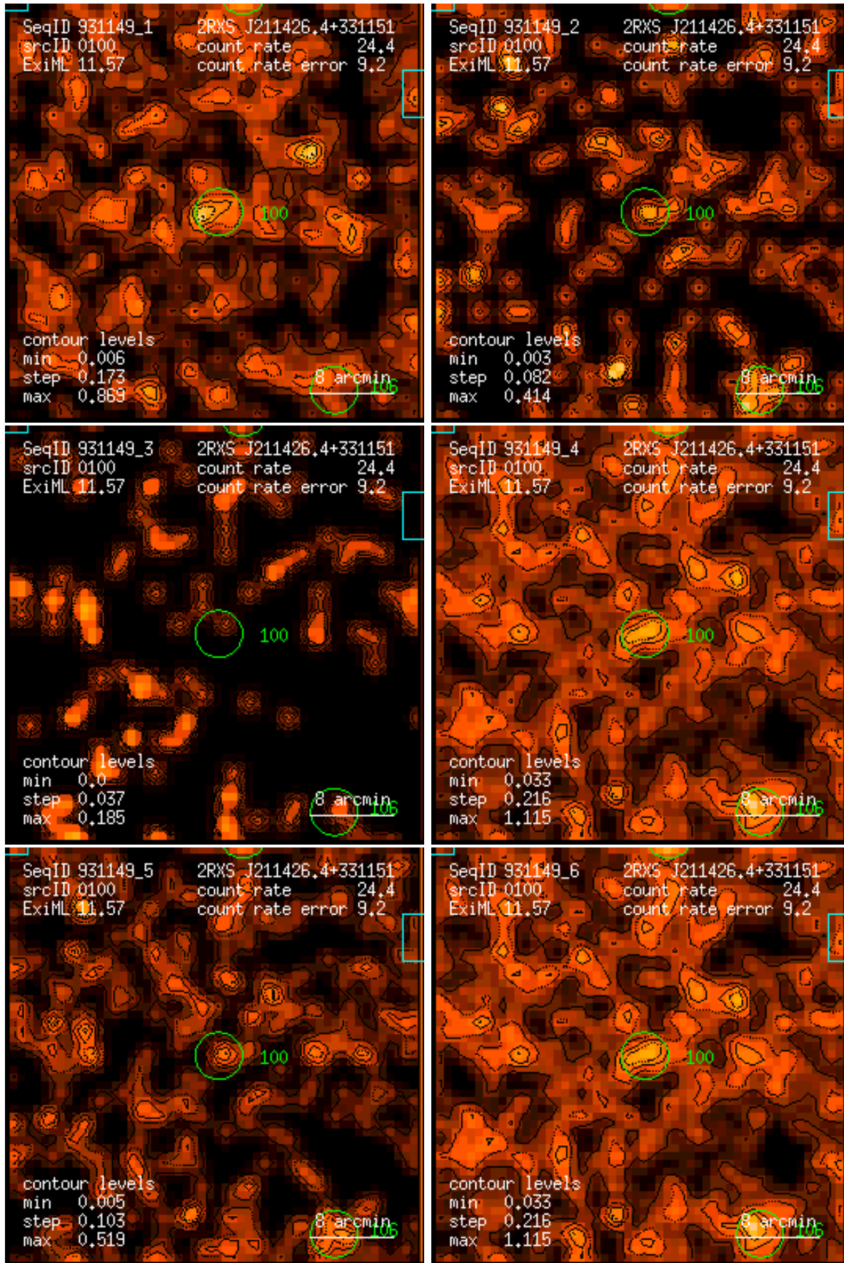
Figure 100: RASS 931149: detection 0100: band rate images, Gaussian filter: (1) PSPC channels 11 – 41, (2) 52 – 90, (3) 91 – 201, (4) 11 – 235, (5) 52 – 201, (6) 11 – 201. Broad band rates in counts/ks. Band rate contour levels in counts/ks/arcmin 2 .
