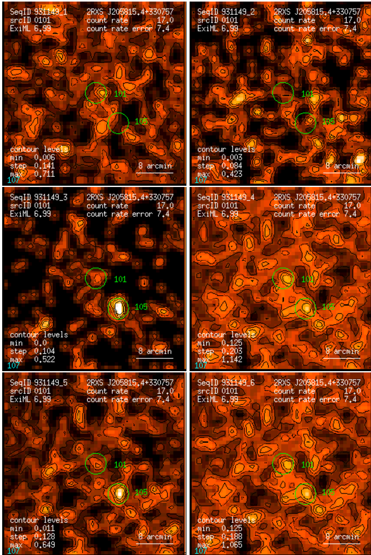
Figure 101: RASS 931149: detection 0101: band rate images, Gaussian filter: (1) PSPC channels 11 – 41, (2) 52 – 90, (3) 91 – 201, (4) 11 – 235, (5) 52 – 201, (6) 11 – 201. Broad band rates in counts/ks. Band rate contour levels in counts/ks/arcmin 2 .
