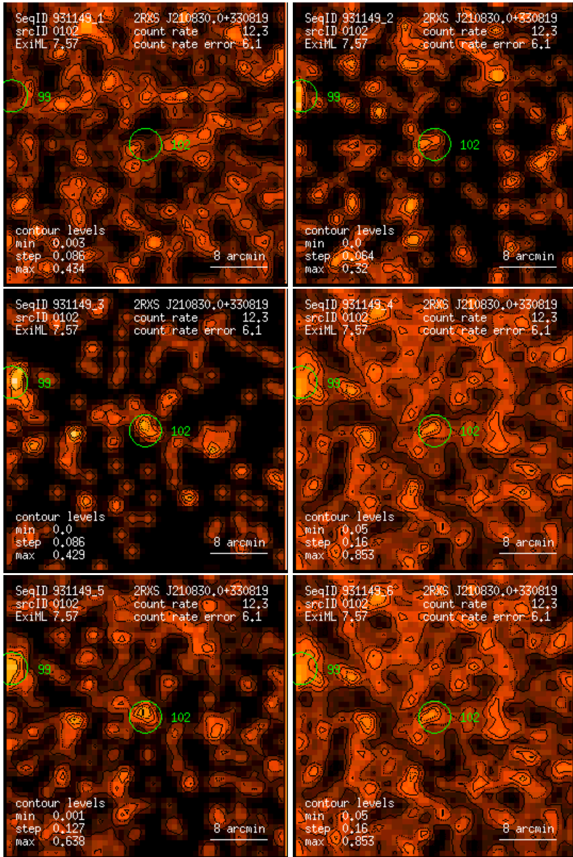
Figure 102: RASS 931149: detection 0102: band rate images, Gaussian filter: (1) PSPC channels 11 – 41, (2) 52 – 90, (3) 91 – 201, (4) 11 – 235, (5) 52 – 201, (6) 11 – 201. Broad band rates in counts/ks. Band rate contour levels in counts/ks/arcmin 2 .
