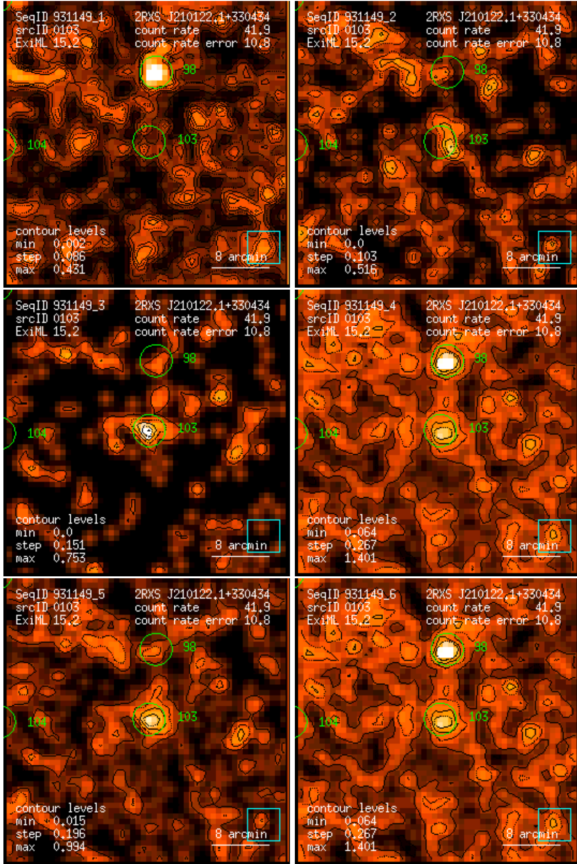
Figure 103: RASS 931149: detection 0103: band rate images, Gaussian filter: (1) PSPC channels 11 – 41, (2) 52 – 90, (3) 91 – 201, (4) 11 – 235, (5) 52 – 201, (6) 11 – 201. Broad band rates in counts/ks. Band rate contour levels in counts/ks/arcmin 2 .
