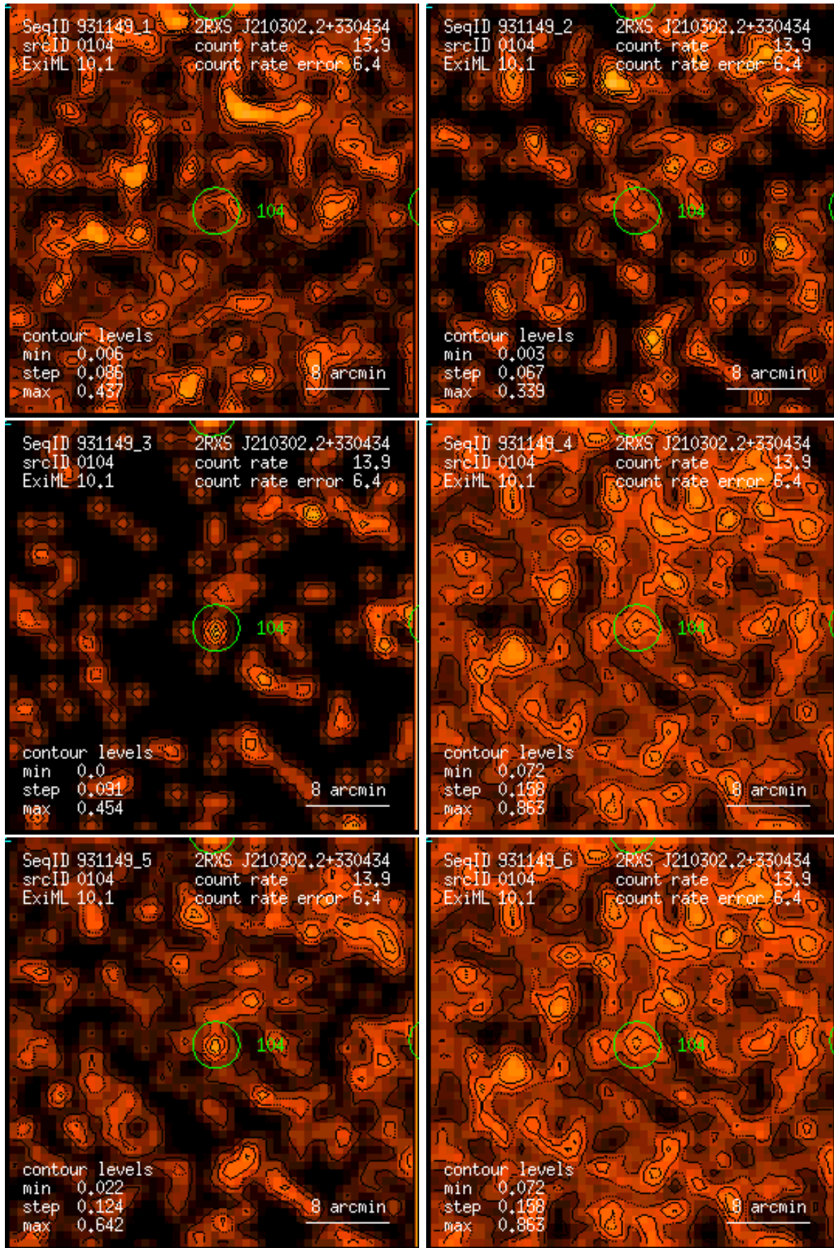
Figure 104: RASS 931149: detection 0104: band rate images, Gaussian filter: (1) PSPC channels 11 – 41, (2) 52 – 90, (3) 91 – 201, (4) 11 – 235, (5) 52 – 201, (6) 11 – 201. Broad band rates in counts/ks. Band rate contour levels in counts/ks/arcmin 2 .
