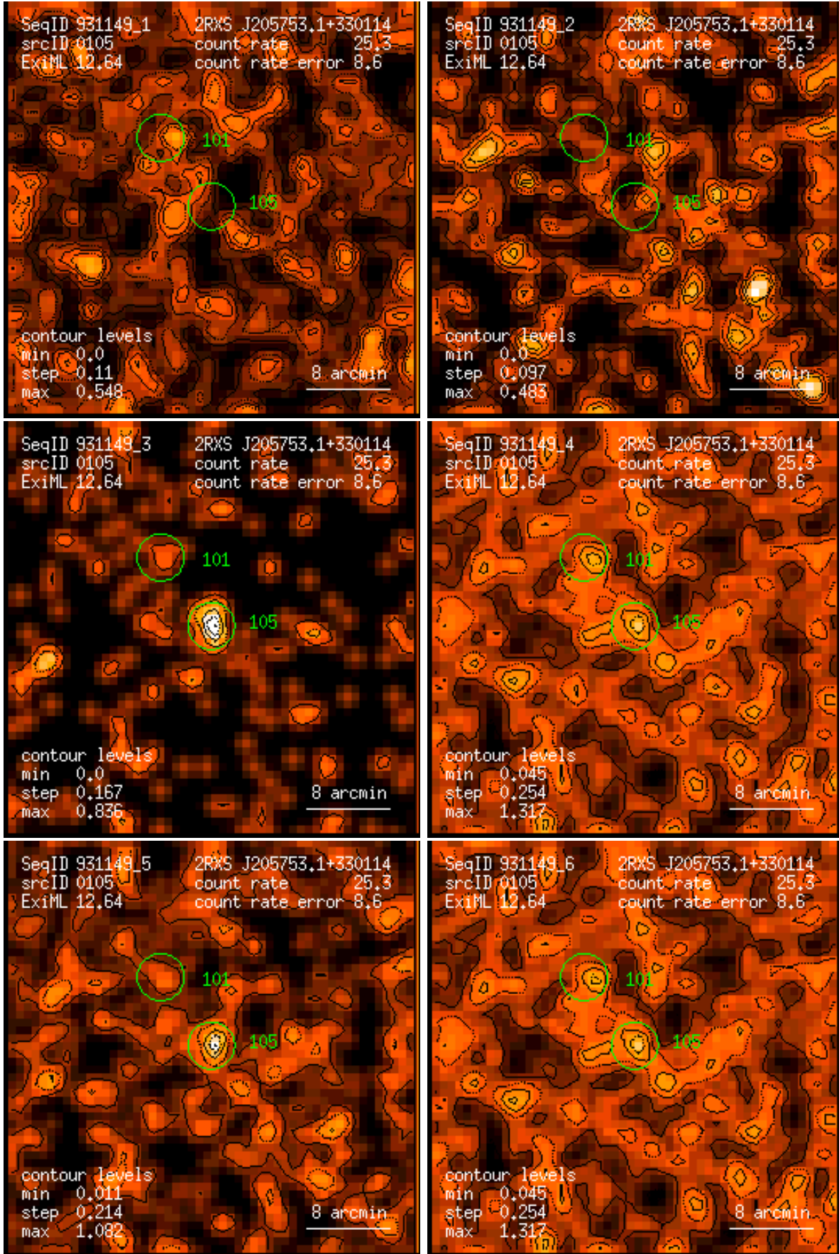
Figure 105: RASS 931149: detection 0105: band rate images, Gaussian filter: (1) PSPC channels 11 – 41, (2) 52 – 90, (3) 91 – 201, (4) 11 – 235, (5) 52 – 201, (6) 11 – 201. Broad band rates in counts/ks. Band rate contour levels in counts/ks/arcmin 2 .
