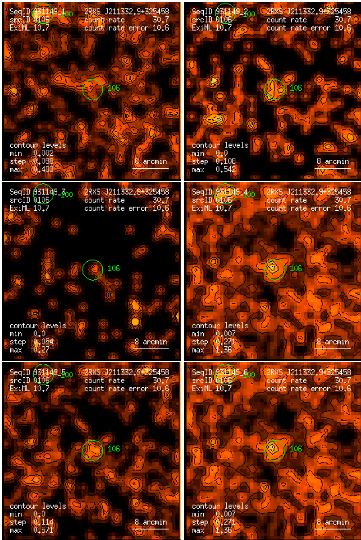
Figure 106: RASS 931149: detection 0106: band rate images, Gaussian filter: (1) PSPC channels 11 – 41, (2) 52 – 90, (3) 91 – 201, (4) 11 – 235, (5) 52 – 201, (6) 11 – 201. Broad band rates in counts/ks. Band rate contour levels in counts/ks/arcmin 2 .
