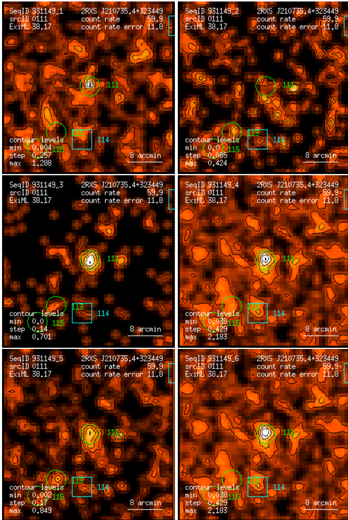
Figure 111: RASS 931149: detection 0111: band rate images, Gaussian filter: (1) PSPC channels 11 – 41, (2) 52 – 90, (3) 91 – 201, (4) 11 – 235, (5) 52 – 201, (6) 11 – 201. Broad band rates in counts/ks. Band rate contour levels in counts/ks/arcmin 2 .
