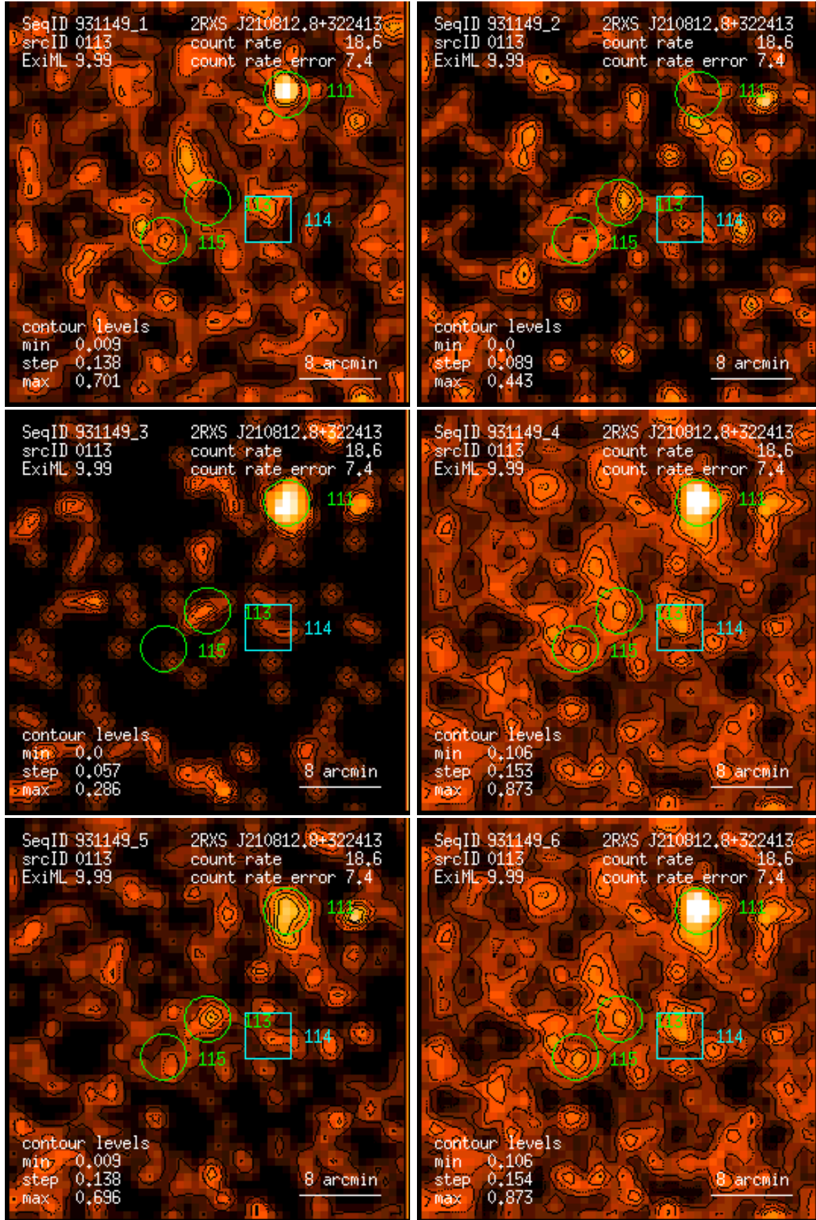
Figure 113: RASS 931149: detection 0113: band rate images, Gaussian filter: (1) PSPC channels 11 – 41, (2) 52 – 90, (3) 91 – 201, (4) 11 – 235, (5) 52 – 201, (6) 11 – 201. Broad band rates in counts/ks. Band rate contour levels in counts/ks/arcmin 2 .
