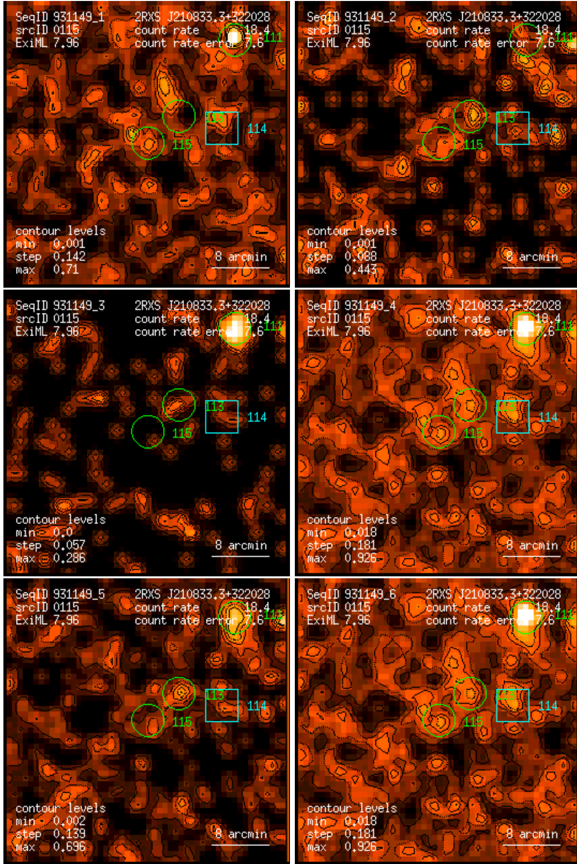
Figure 115: RASS 931149: detection 0115: band rate images, Gaussian filter: (1) PSPC channels 11 – 41, (2) 52 – 90, (3) 91 – 201, (4) 11 – 235, (5) 52 – 201, (6) 11 – 201. Broad band rates in counts/ks. Band rate contour levels in counts/ks/arcmin 2 .
