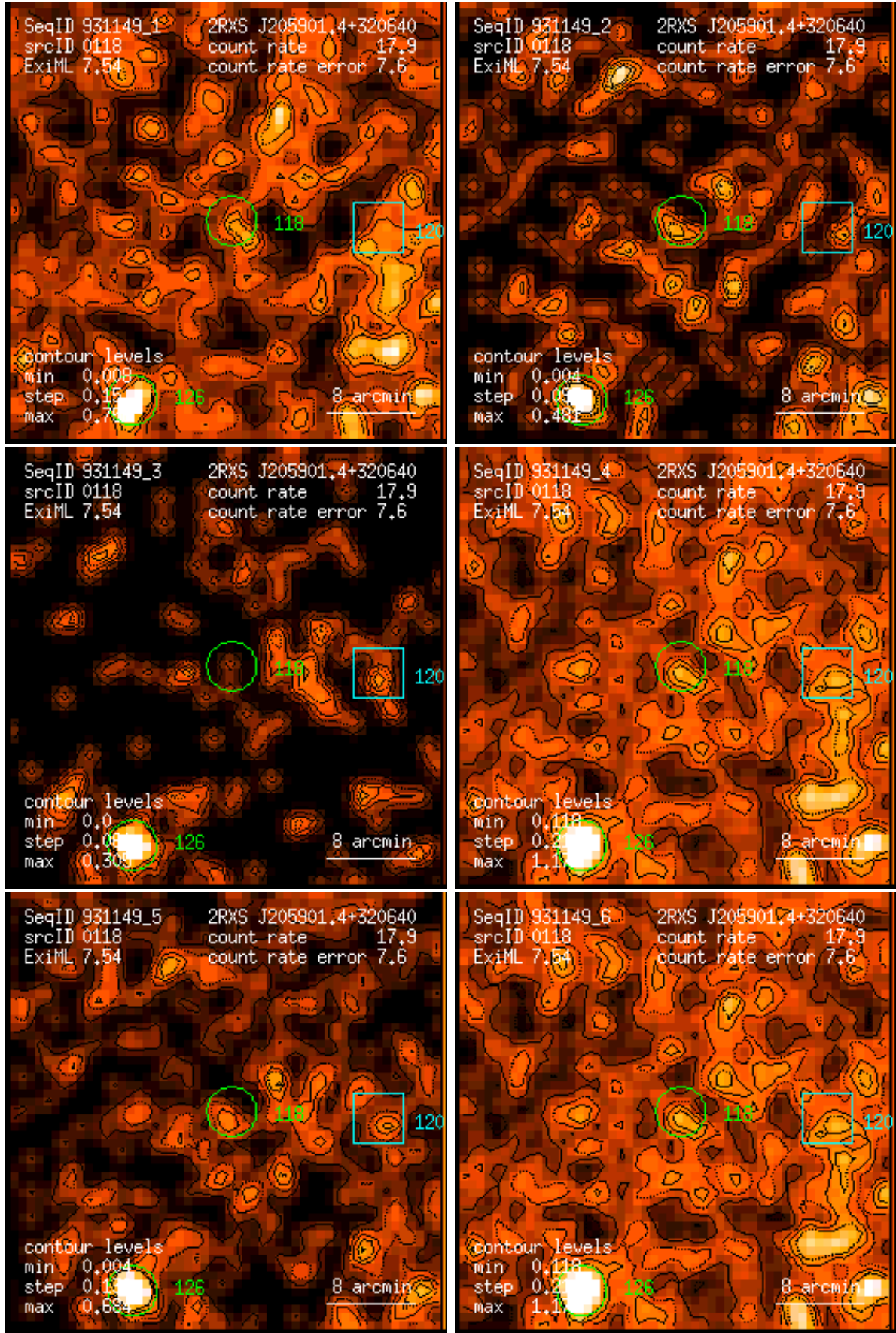
Figure 118: RASS 931149: detection 0118: band rate images, Gaussian filter: (1) PSPC channels 11 – 41, (2) 52 – 90, (3) 91 – 201, (4) 11 – 235, (5) 52 – 201, (6) 11 – 201. Broad band rates in counts/ks. Band rate contour levels in counts/ks/arcmin 2 .
