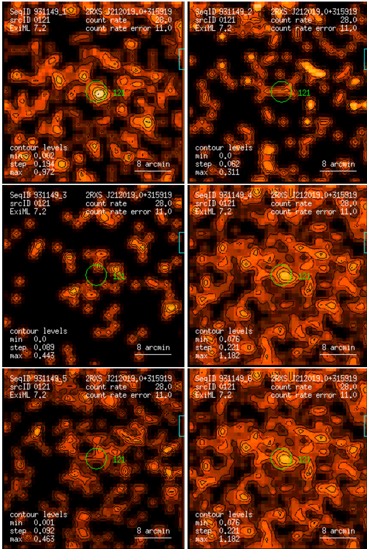
Figure 121: RASS 931149: detection 0121: band rate images, Gaussian filter: (1) PSPC channels 11 – 41, (2) 52 – 90, (3) 91 – 201, (4) 11 – 235, (5) 52 – 201, (6) 11 – 201. Broad band rates in counts/ks. Band rate contour levels in counts/ks/arcmin 2 .
