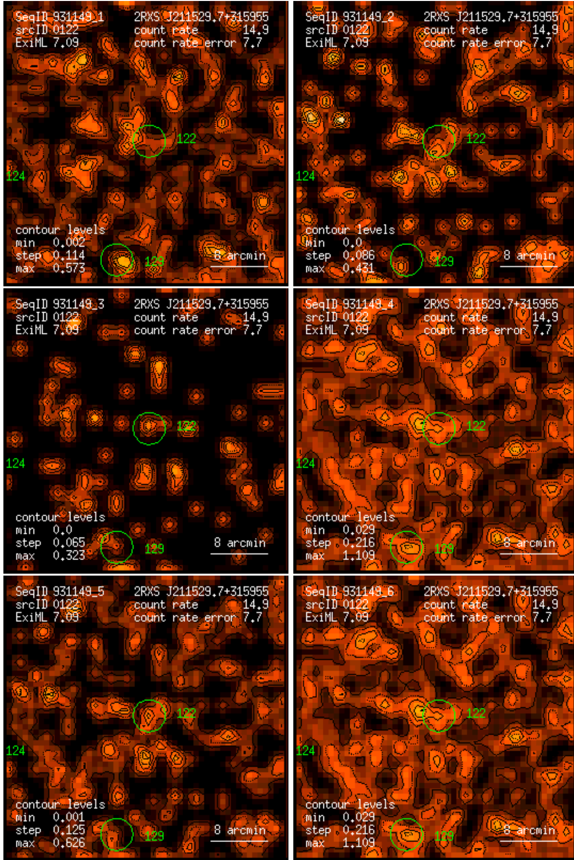
Figure 122: RASS 931149: detection 0122: band rate images, Gaussian filter: (1) PSPC channels 11 – 41, (2) 52 – 90, (3) 91 – 201, (4) 11 – 235, (5) 52 – 201, (6) 11 – 201. Broad band rates in counts/ks. Band rate contour levels in counts/ks/arcmin 2 .
