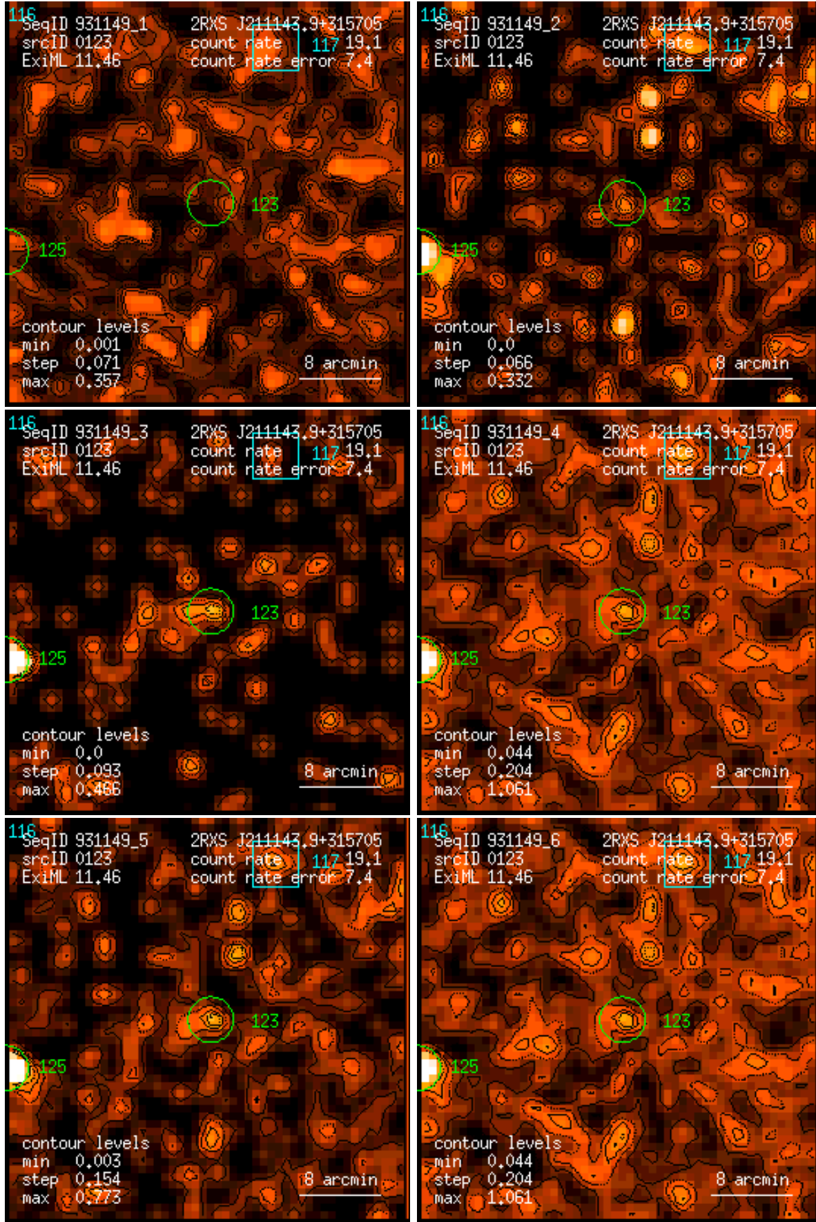
Figure 123: RASS 931149: detection 0123: band rate images, Gaussian filter: (1) PSPC channels 11 – 41, (2) 52 – 90, (3) 91 – 201, (4) 11 – 235, (5) 52 – 201, (6) 11 – 201. Broad band rates in counts/ks. Band rate contour levels in counts/ks/arcmin 2 .
