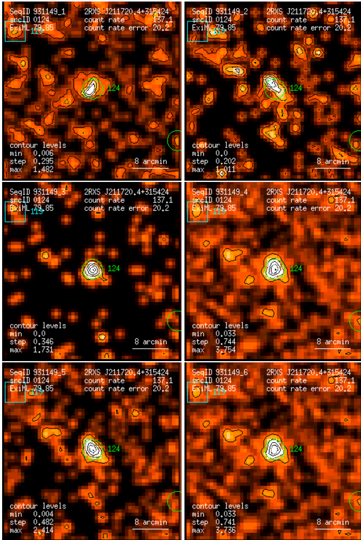
Figure 124: RASS 931149: detection 0124: band rate images, Gaussian filter: (1) PSPC channels 11 – 41, (2) 52 – 90, (3) 91 – 201, (4) 11 – 235, (5) 52 – 201, (6) 11 – 201. Broad band rates in counts/ks. Band rate contour levels in counts/ks/arcmin 2 .
