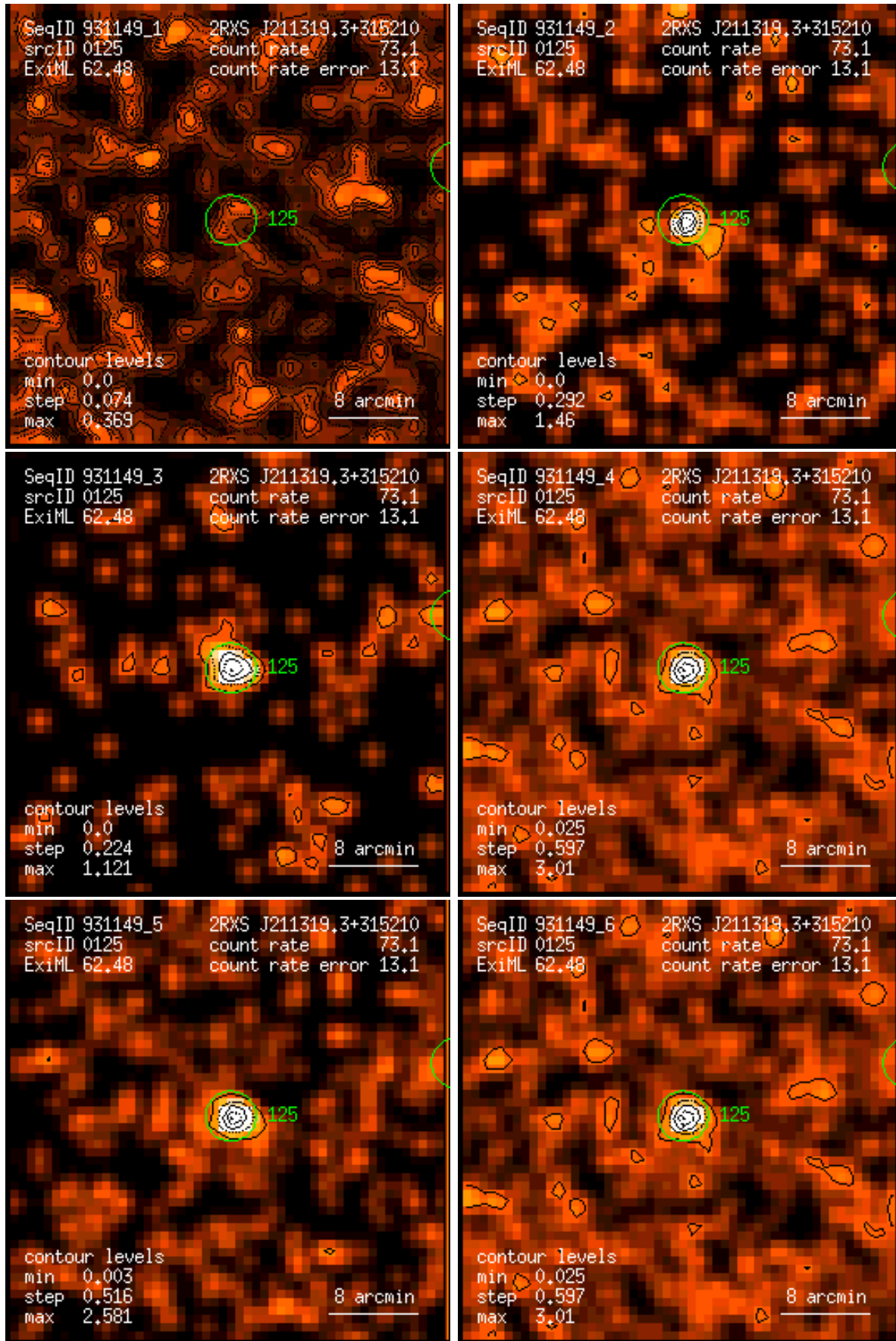
Figure 125: RASS 931149: detection 0125: band rate images, Gaussian filter: (1) PSPC channels 11 – 41, (2) 52 – 90, (3) 91 – 201, (4) 11 – 235, (5) 52 – 201, (6) 11 – 201. Broad band rates in counts/ks. Band rate contour levels in counts/ks/arcmin 2 .
