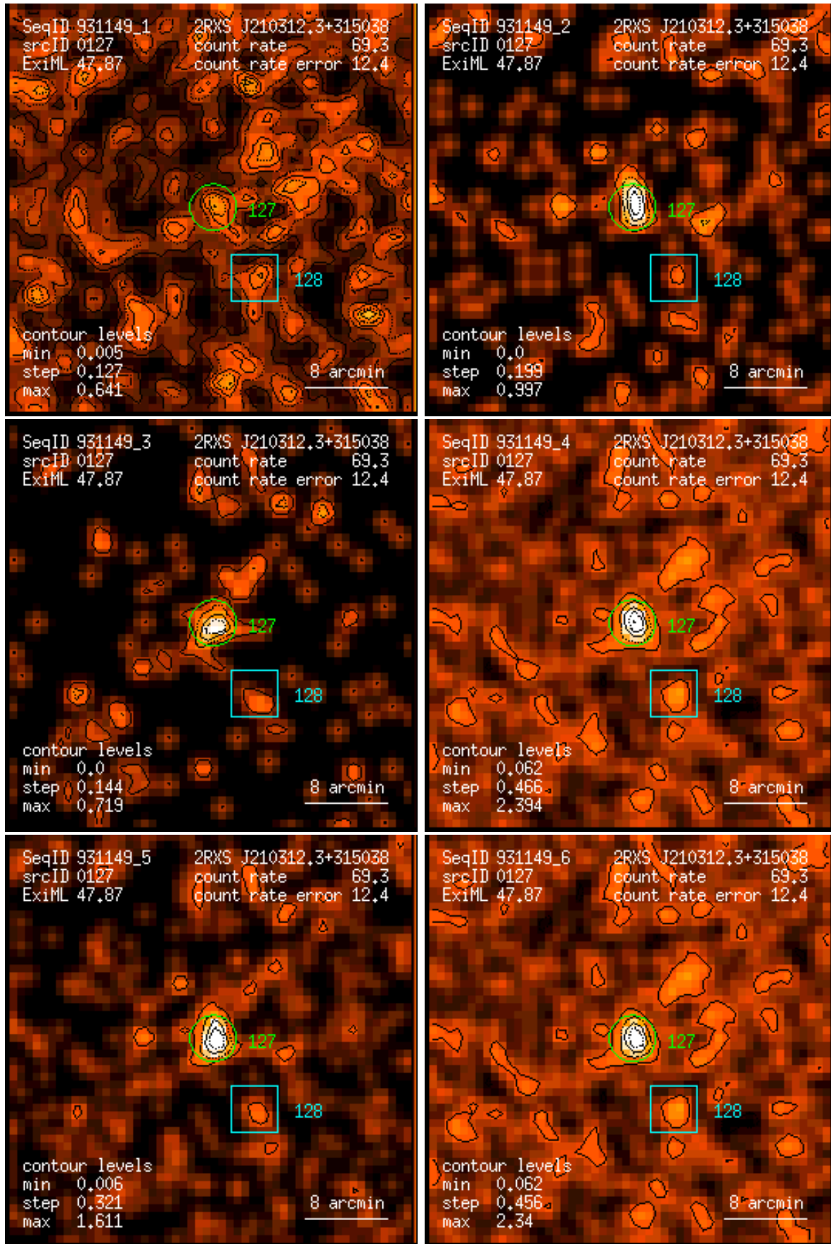
Figure 127: RASS 931149: detection 0127: band rate images, Gaussian filter: (1) PSPC channels 11 – 41, (2) 52 – 90, (3) 91 – 201, (4) 11 – 235, (5) 52 – 201, (6) 11 – 201. Broad band rates in counts/ks. Band rate contour levels in counts/ks/arcmin 2 .
