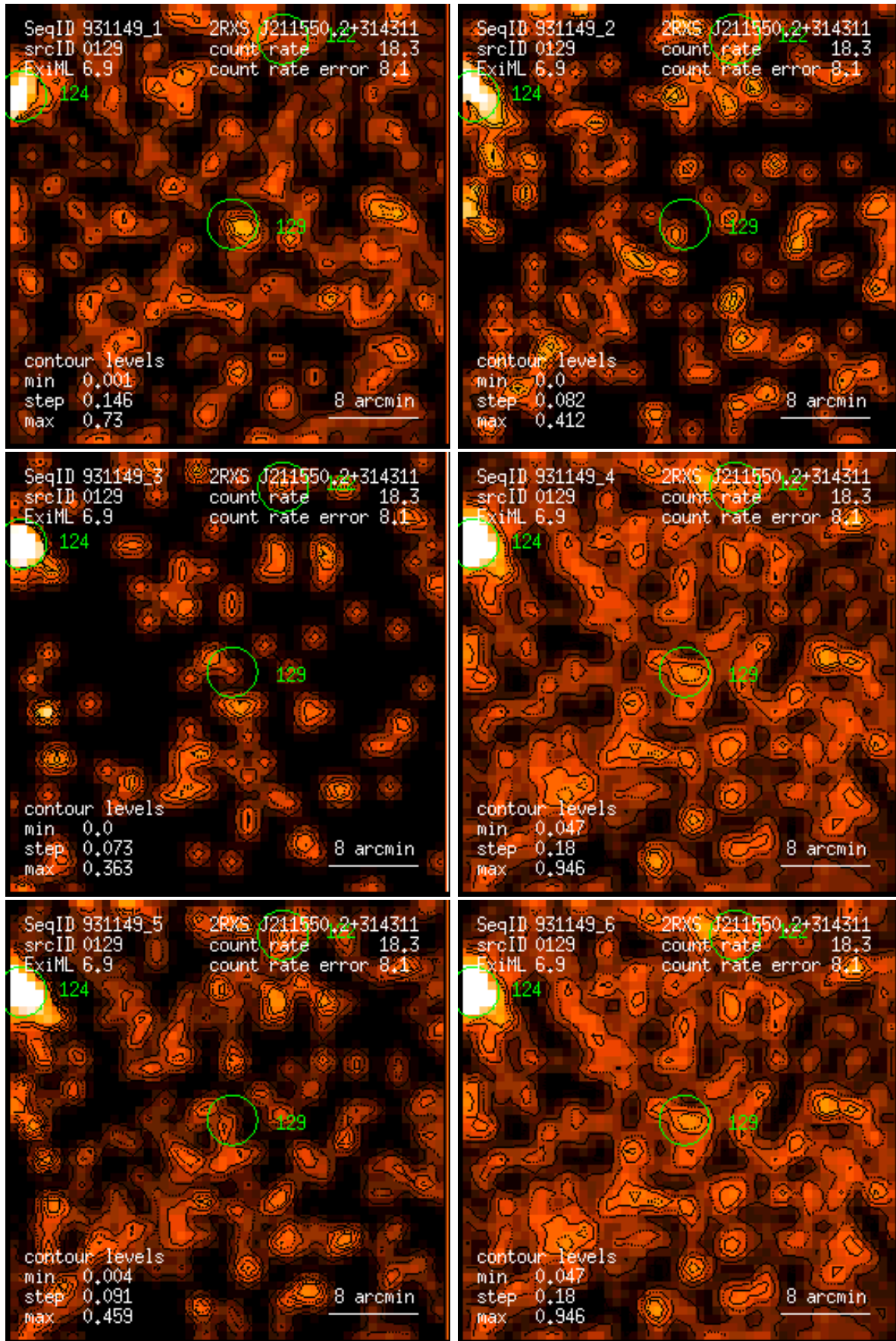
Figure 129: RASS 931149: detection 0129: band rate images, Gaussian filter: (1) PSPC channels 11 – 41, (2) 52 – 90, (3) 91 – 201, (4) 11 – 235, (5) 52 – 201, (6) 11 – 201. Broad band rates in counts/ks. Band rate contour levels in counts/ks/arcmin 2 .
