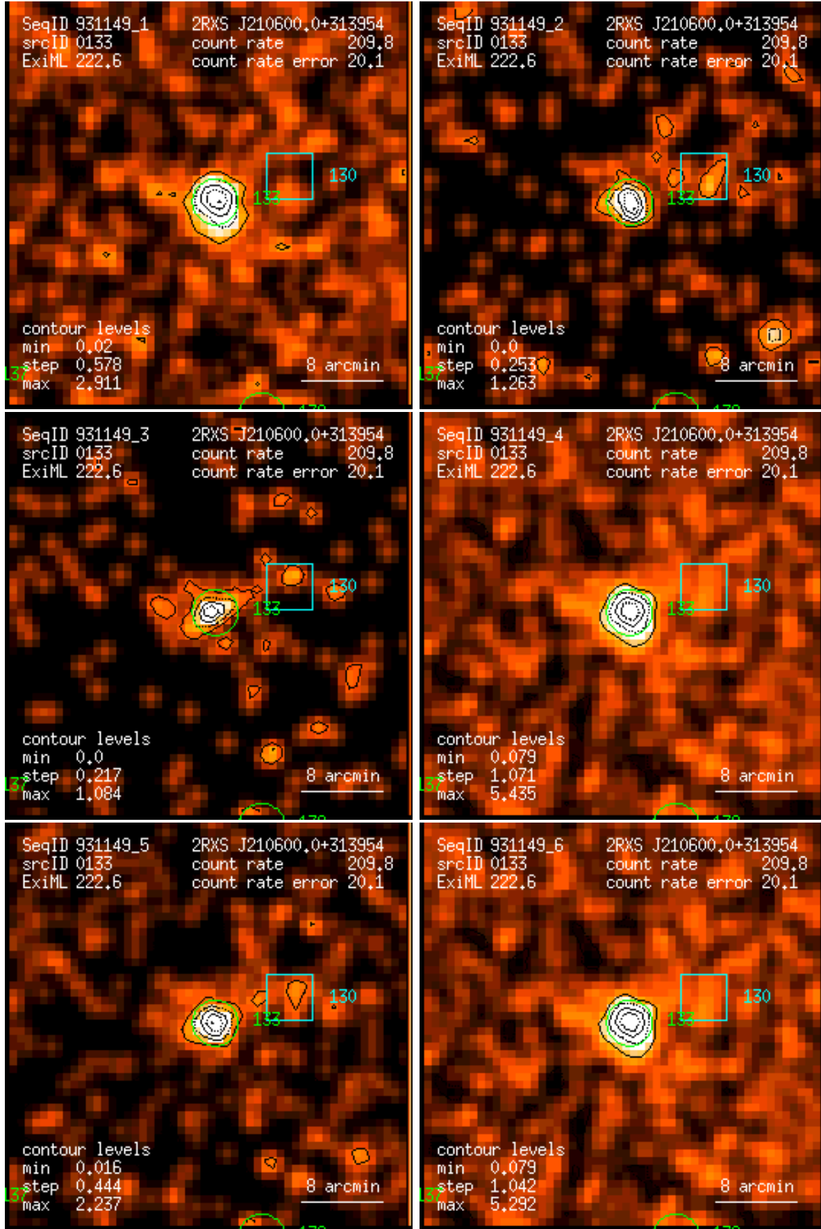
Figure 133: RASS 931149: detection 0133: band rate images, Gaussian filter: (1) PSPC channels 11 – 41, (2) 52 – 90, (3) 91 – 201, (4) 11 – 235, (5) 52 – 201, (6) 11 – 201. Broad band rates in counts/ks. Band rate contour levels in counts/ks/arcmin 2 .
