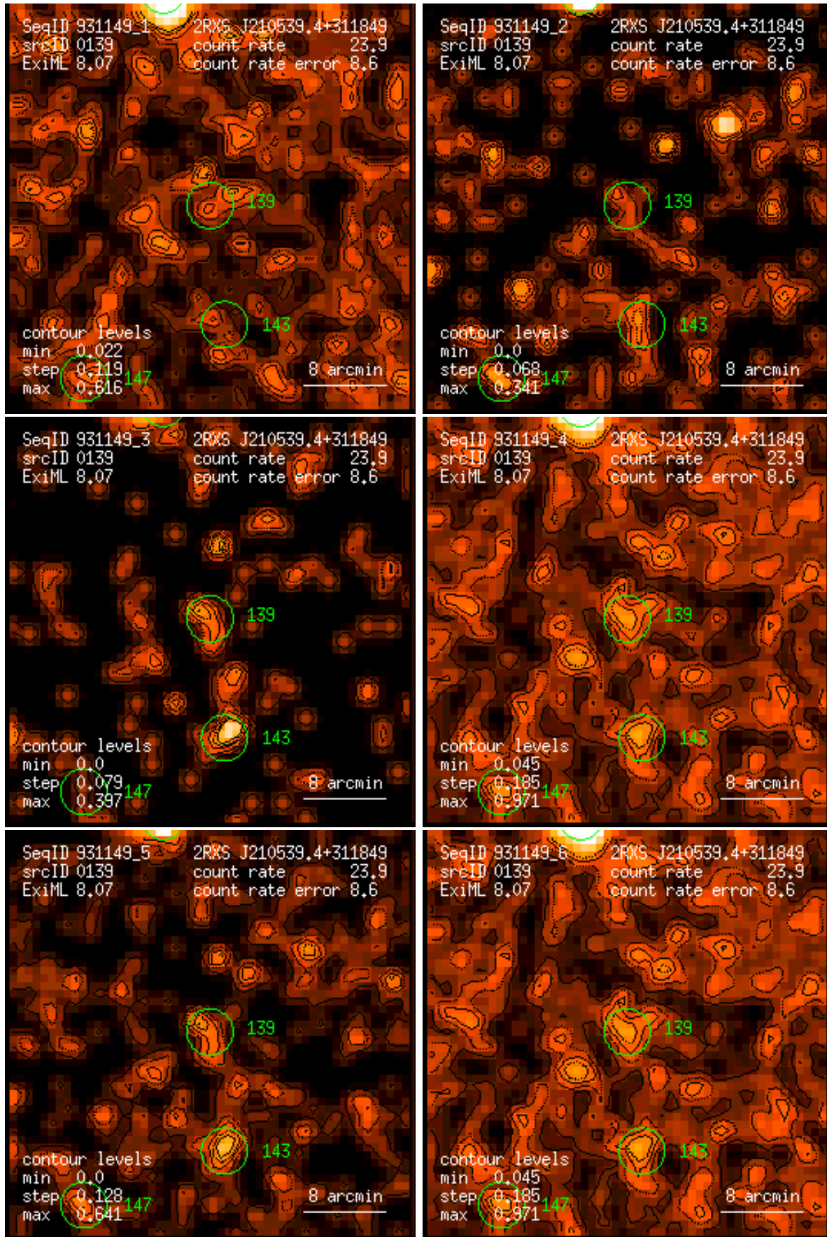
Figure 139: RASS 931149: detection 0139: band rate images, Gaussian filter: (1) PSPC channels 11 – 41, (2) 52 – 90, (3) 91 – 201, (4) 11 – 235, (5) 52 – 201, (6) 11 – 201. Broad band rates in counts/ks. Band rate contour levels in counts/ks/arcmin 2 .
