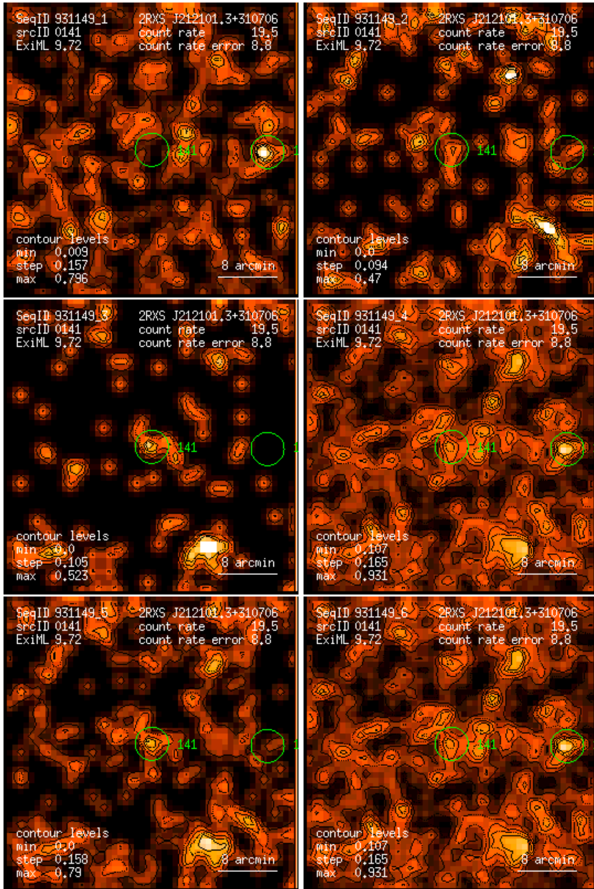
Figure 141: RASS 931149: detection 0141: band rate images, Gaussian filter: (1) PSPC channels 11 – 41, (2) 52 – 90, (3) 91 – 201, (4) 11 – 235, (5) 52 – 201, (6) 11 – 201. Broad band rates in counts/ks. Band rate contour levels in counts/ks/arcmin 2 .
