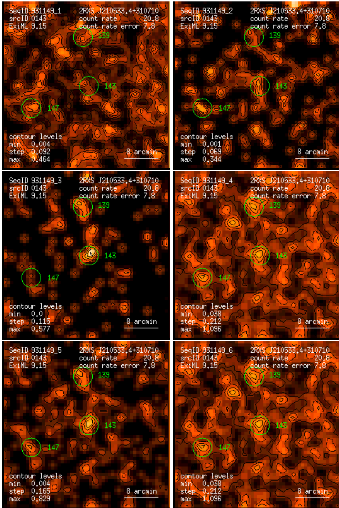
Figure 143: RASS 931149: detection 0143: band rate images, Gaussian filter: (1) PSPC channels 11 – 41, (2) 52 – 90, (3) 91 – 201, (4) 11 – 235, (5) 52 – 201, (6) 11 – 201. Broad band rates in counts/ks. Band rate contour levels in counts/ks/arcmin 2 .
