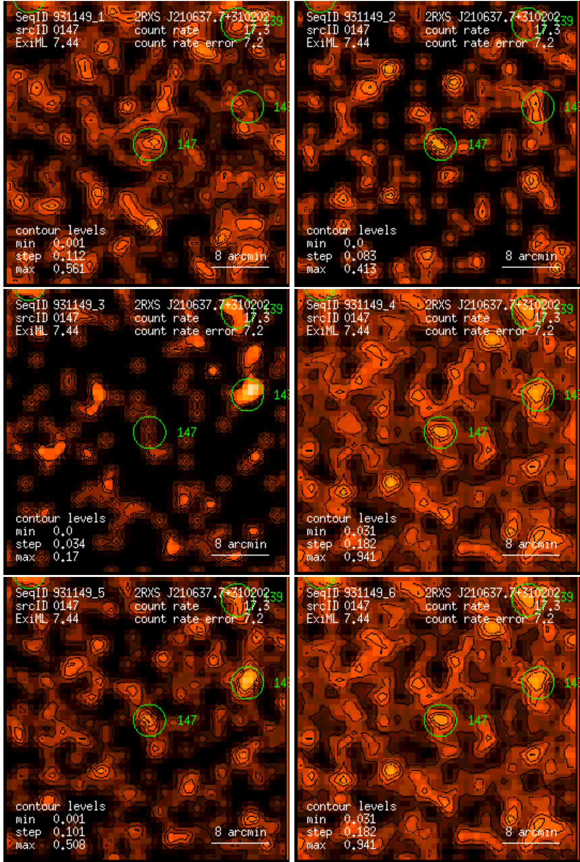
Figure 147: RASS 931149: detection 0147: band rate images, Gaussian filter: (1) PSPC channels 11 – 41, (2) 52 – 90, (3) 91 – 201, (4) 11 – 235, (5) 52 – 201, (6) 11 – 201. Broad band rates in counts/ks. Band rate contour levels in counts/ks/arcmin 2 .
