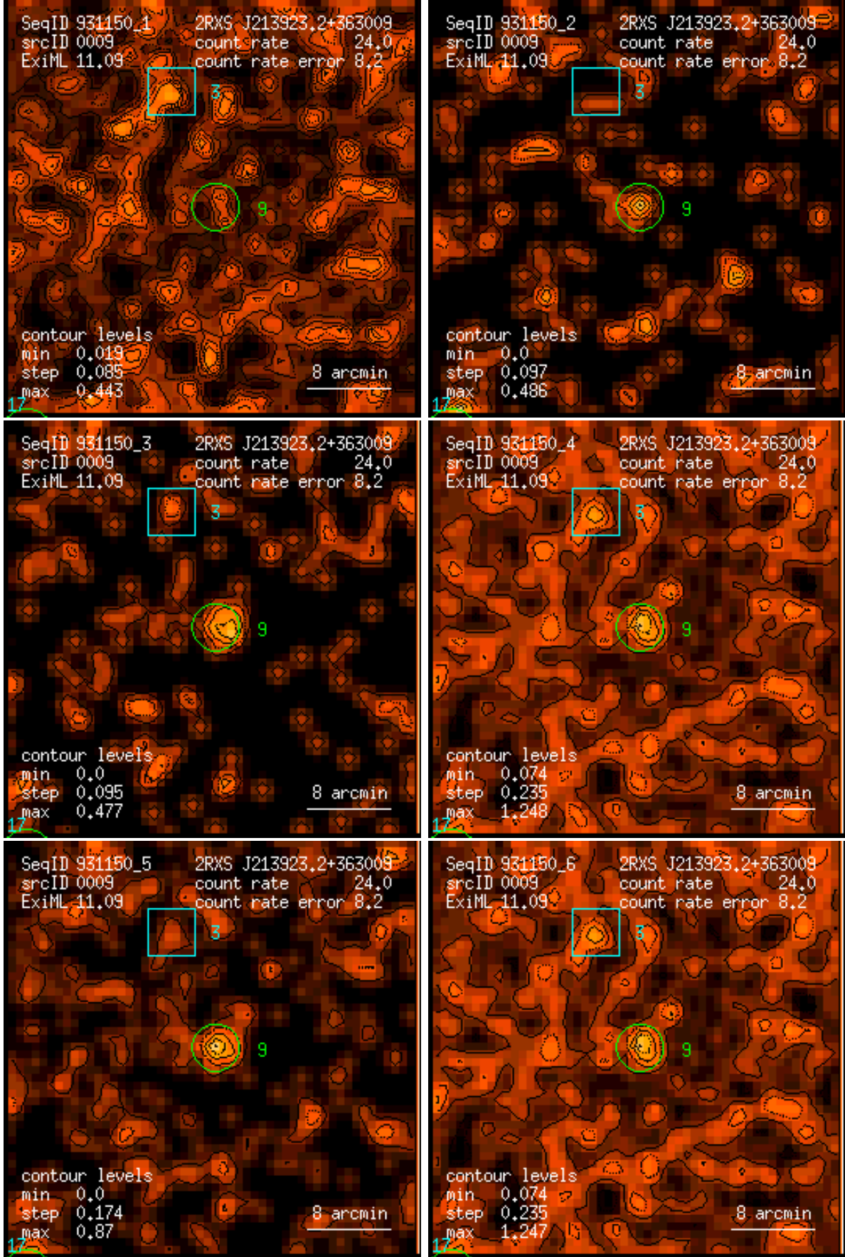
Figure 9: RASS 931150: detection 0009: band rate images, Gaussian filter: (1) PSPC channels 11 – 41, (2) 52 – 90, (3) 91 – 201, (4) 11 – 235, (5) 52 – 201, (6) 11 – 201. Broad band rates in counts/ks. Band rate contour levels in counts/ks/arcmin 2 .
