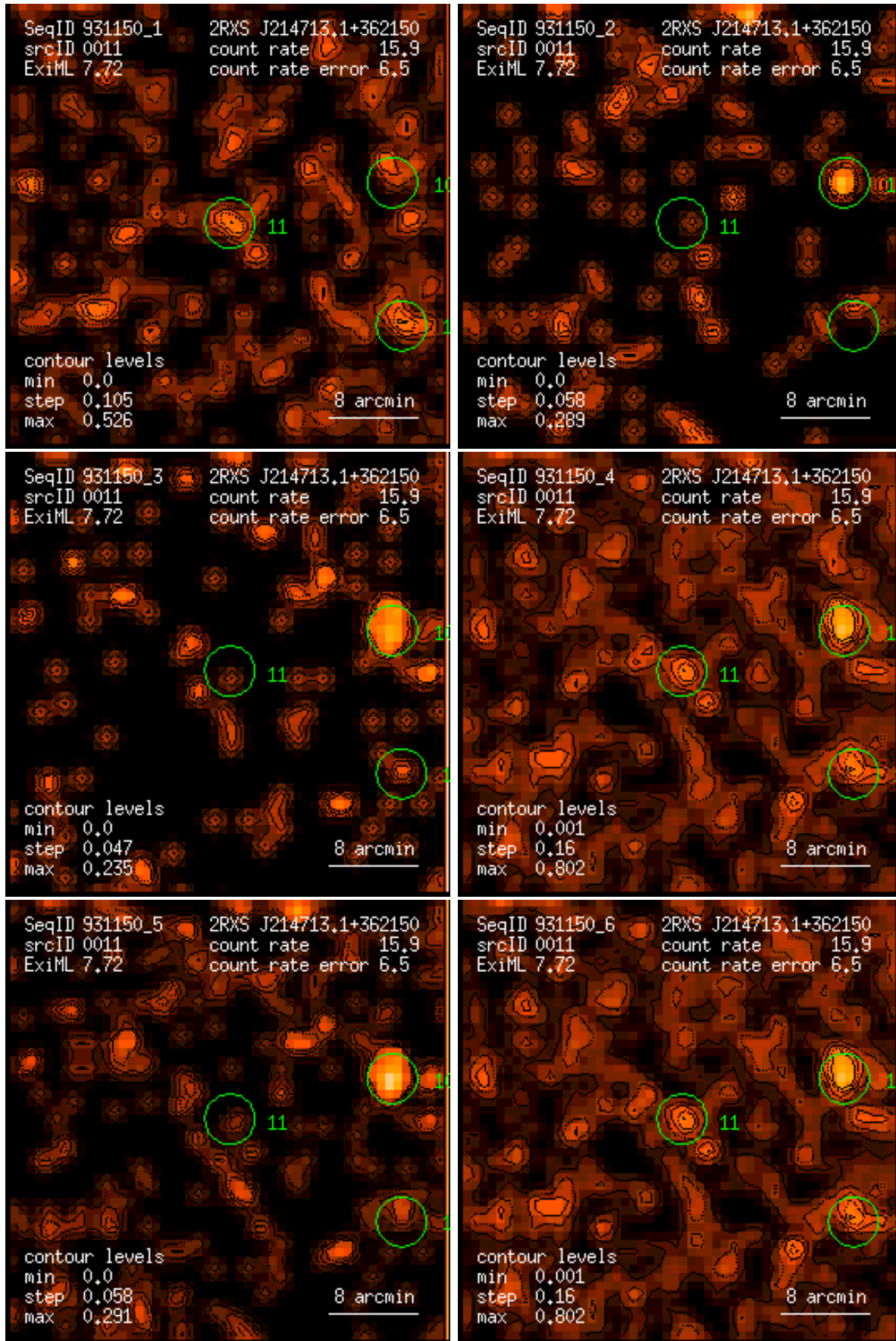
Figure 11: RASS 931150: detection 0011: band rate images, Gaussian filter: (1) PSPC channels 11 – 41, (2) 52 – 90, (3) 91 – 201, (4) 11 – 235, (5) 52 – 201, (6) 11 – 201. Broad band rates in counts/ks. Band rate contour levels in counts/ks/arcmin 2 .
