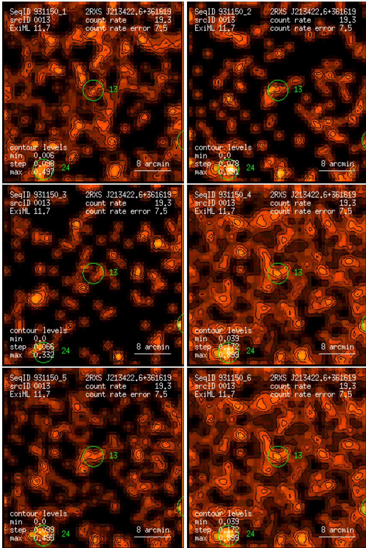
Figure 13: RASS 931150: detection 0013: band rate images, Gaussian filter: (1) PSPC channels 11 – 41, (2) 52 – 90, (3) 91 – 201, (4) 11 – 235, (5) 52 – 201, (6) 11 – 201. Broad band rates in counts/ks. Band rate contour levels in counts/ks/arcmin 2 .
