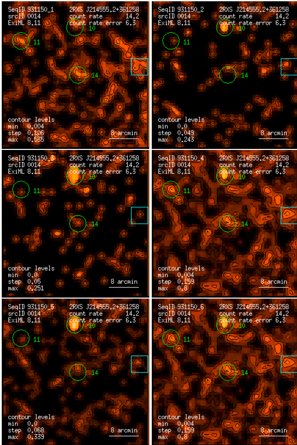
Figure 14: RASS 931150: detection 0014: band rate images, Gaussian filter: (1) PSPC channels 11 – 41, (2) 52 – 90, (3) 91 – 201, (4) 11 – 235, (5) 52 – 201, (6) 11 – 201. Broad band rates in counts/ks. Band rate contour levels in counts/ks/arcmin 2 .
