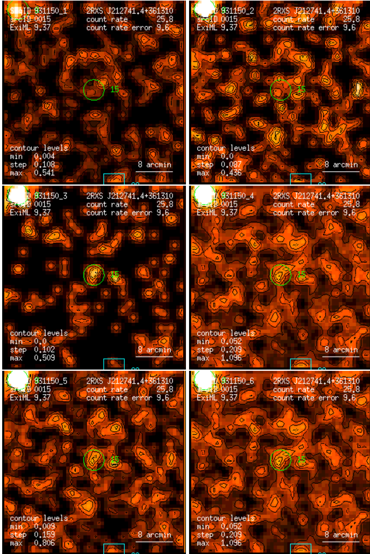
Figure 15: RASS 931150: detection 0015: band rate images, Gaussian filter: (1) PSPC channels 11 – 41, (2) 52 – 90, (3) 91 – 201, (4) 11 – 235, (5) 52 – 201, (6) 11 – 201. Broad band rates in counts/ks. Band rate contour levels in counts/ks/arcmin 2 .
