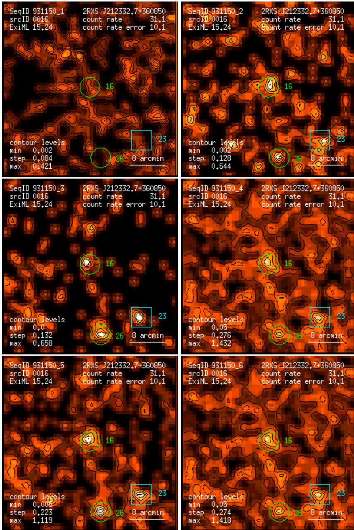
Figure 16: RASS 931150: detection 0016: band rate images, Gaussian filter: (1) PSPC channels 11 – 41, (2) 52 – 90, (3) 91 – 201, (4) 11 – 235, (5) 52 – 201, (6) 11 – 201. Broad band rates in counts/ks. Band rate contour levels in counts/ks/arcmin 2 .
