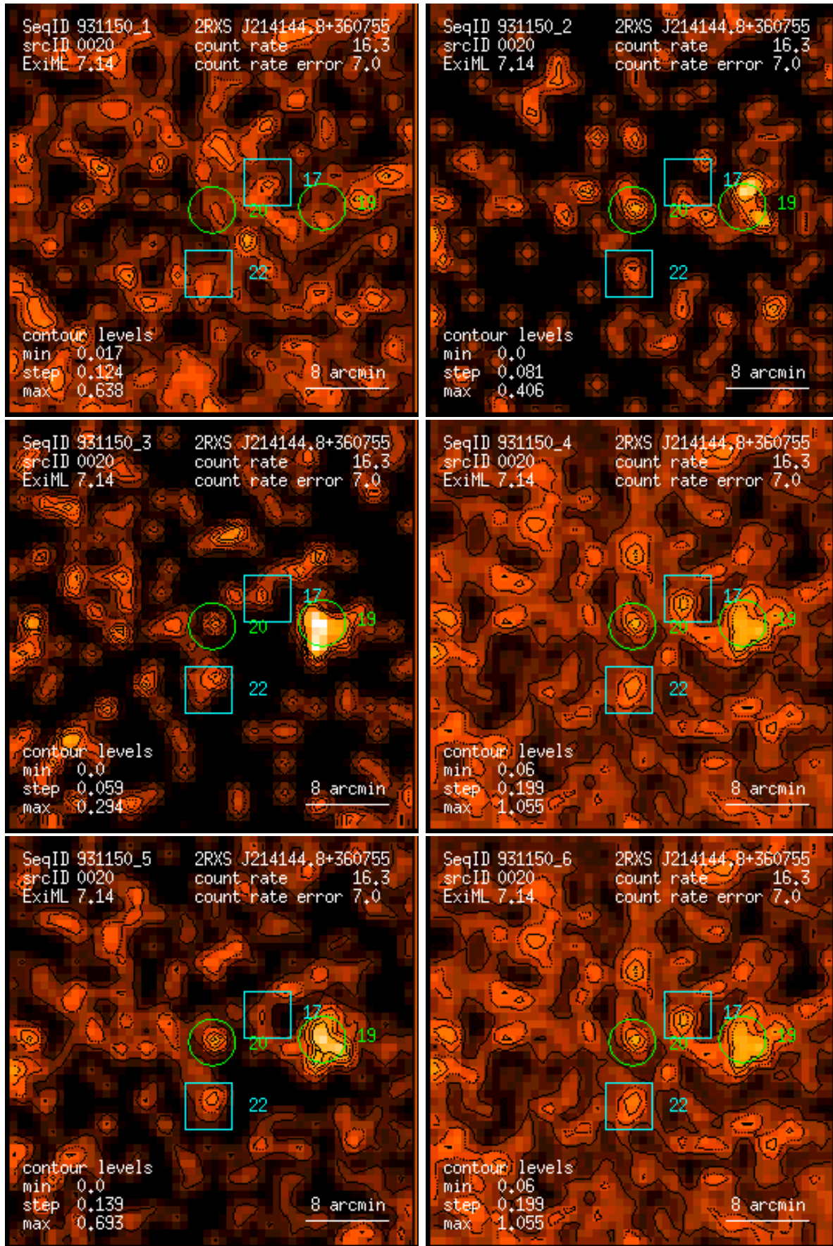
Figure 20: RASS 931150: detection 0020: band rate images, Gaussian filter: (1) PSPC channels 11 – 41, (2) 52 – 90, (3) 91 – 201, (4) 11 – 235, (5) 52 – 201, (6) 11 – 201. Broad band rates in counts/ks. Band rate contour levels in counts/ks/arcmin 2 .
