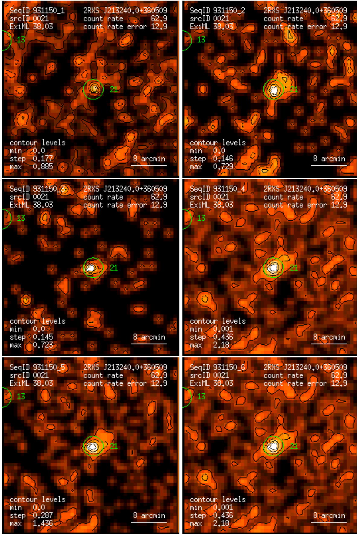
Figure 21: RASS 931150: detection 0021: band rate images, Gaussian filter: (1) PSPC channels 11 – 41, (2) 52 – 90, (3) 91 – 201, (4) 11 – 235, (5) 52 – 201, (6) 11 – 201. Broad band rates in counts/ks. Band rate contour levels in counts/ks/arcmin 2 .
