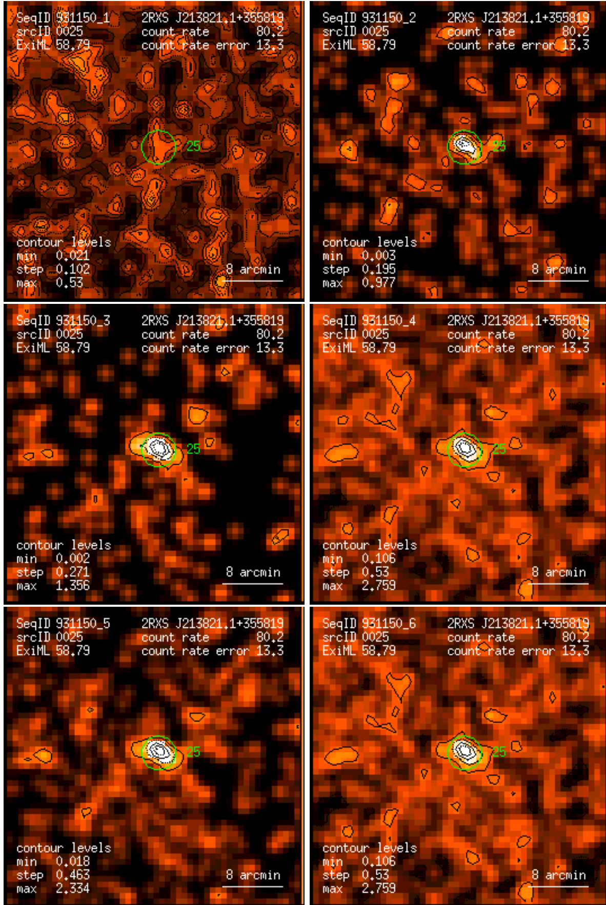
Figure 25: RASS 931150: detection 0025: band rate images, Gaussian filter: (1) PSPC channels 11 – 41, (2) 52 – 90, (3) 91 – 201, (4) 11 – 235, (5) 52 – 201, (6) 11 – 201. Broad band rates in counts/ks. Band rate contour levels in counts/ks/arcmin 2 .
