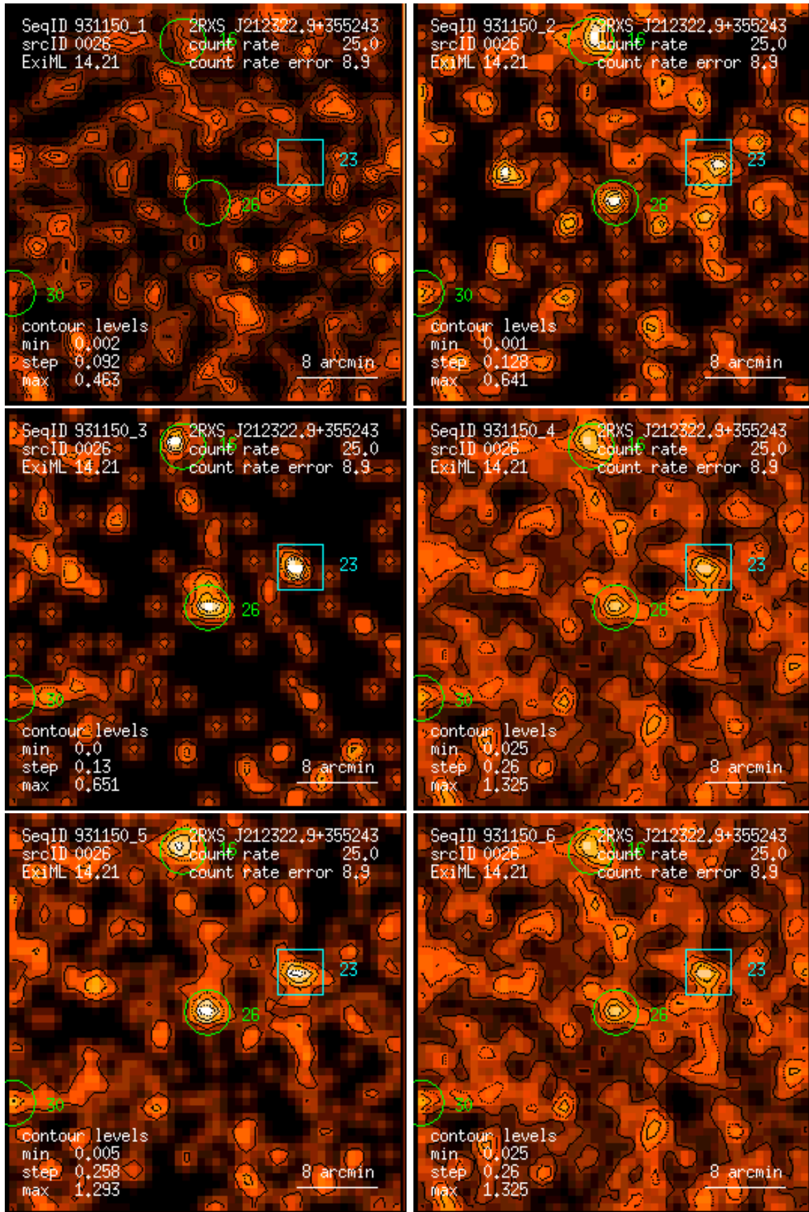
Figure 26: RASS 931150: detection 0026: band rate images, Gaussian filter: (1) PSPC channels 11 – 41, (2) 52 – 90, (3) 91 – 201, (4) 11 – 235, (5) 52 – 201, (6) 11 – 201. Broad band rates in counts/ks. Band rate contour levels in counts/ks/arcmin 2 .
