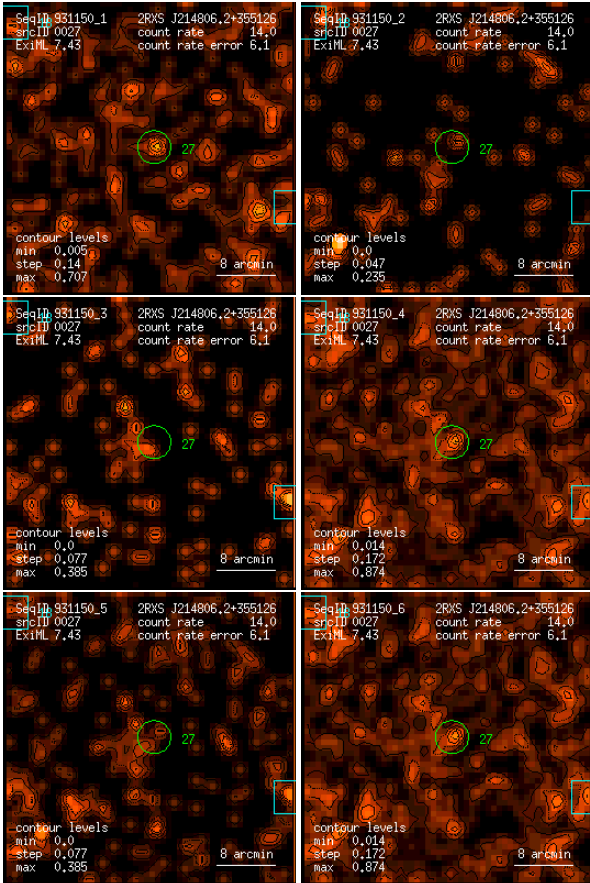
Figure 27: RASS 931150: detection 0027: band rate images, Gaussian filter: (1) PSPC channels 11 – 41, (2) 52 – 90, (3) 91 – 201, (4) 11 – 235, (5) 52 – 201, (6) 11 – 201. Broad band rates in counts/ks. Band rate contour levels in counts/ks/arcmin 2 .
