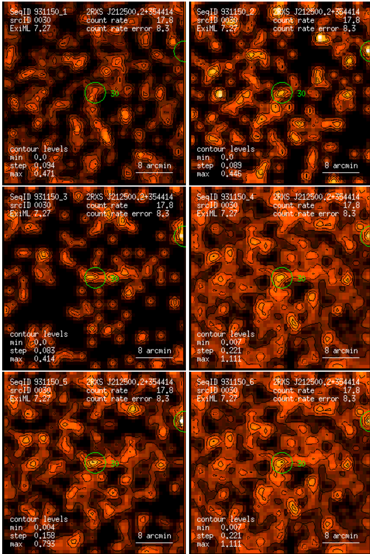
Figure 30: RASS 931150: detection 0030: band rate images, Gaussian filter: (1) PSPC channels 11 – 41, (2) 52 – 90, (3) 91 – 201, (4) 11 – 235, (5) 52 – 201, (6) 11 – 201. Broad band rates in counts/ks. Band rate contour levels in counts/ks/arcmin 2 .
