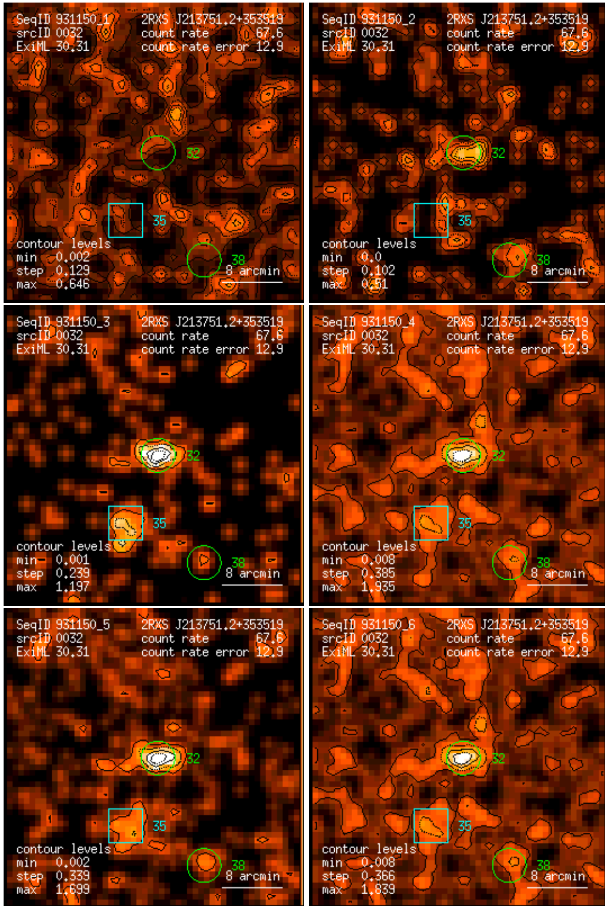
Figure 32: RASS 931150: detection 0032: band rate images, Gaussian filter: (1) PSPC channels 11 – 41, (2) 52 – 90, (3) 91 – 201, (4) 11 – 235, (5) 52 – 201, (6) 11 – 201. Broad band rates in counts/ks. Band rate contour levels in counts/ks/arcmin 2 .
