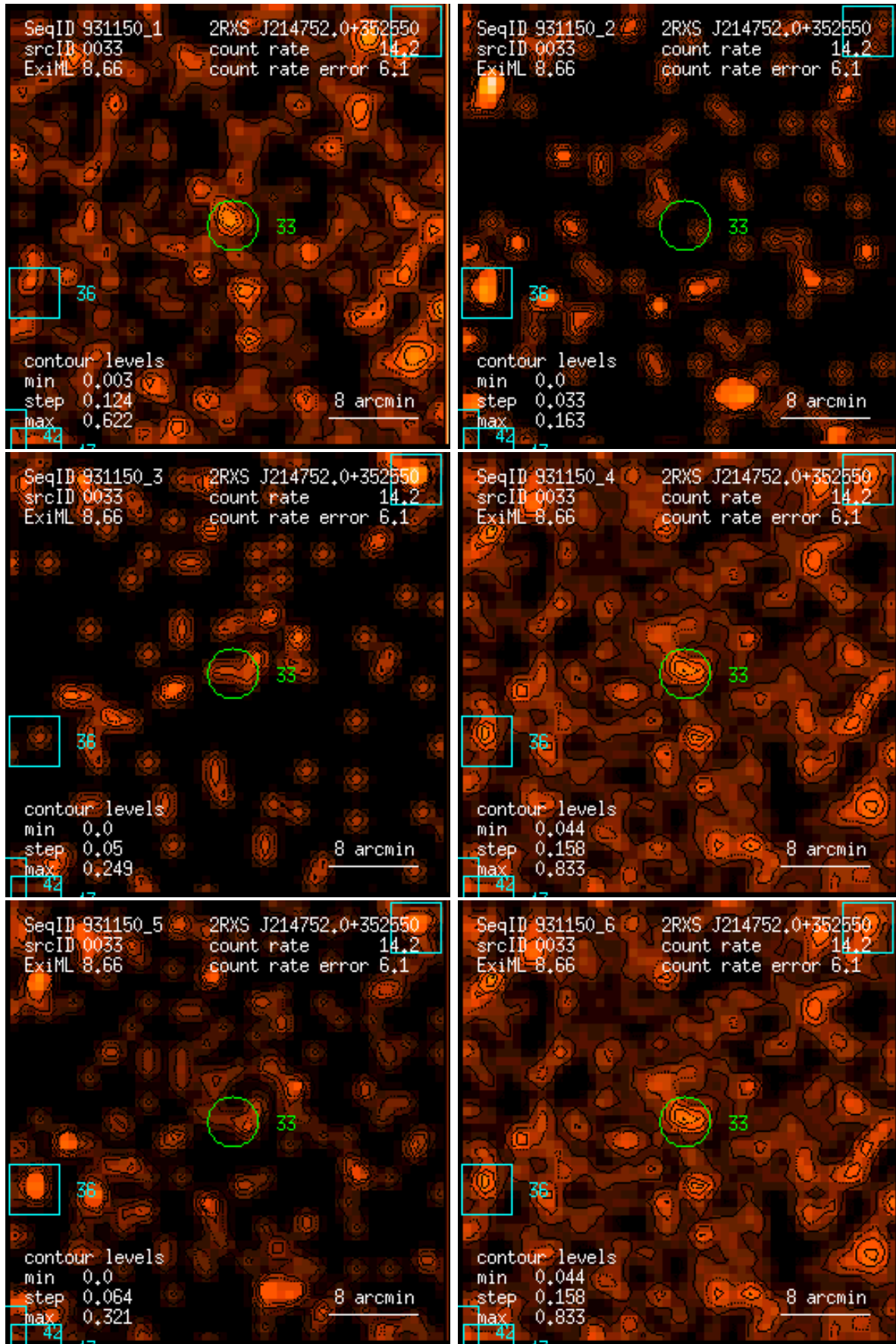
Figure 33: RASS 931150: detection 0033: band rate images, Gaussian filter: (1) PSPC channels 11 – 41, (2) 52 – 90, (3) 91 – 201, (4) 11 – 235, (5) 52 – 201, (6) 11 – 201. Broad band rates in counts/ks. Band rate contour levels in counts/ks/arcmin 2 .
