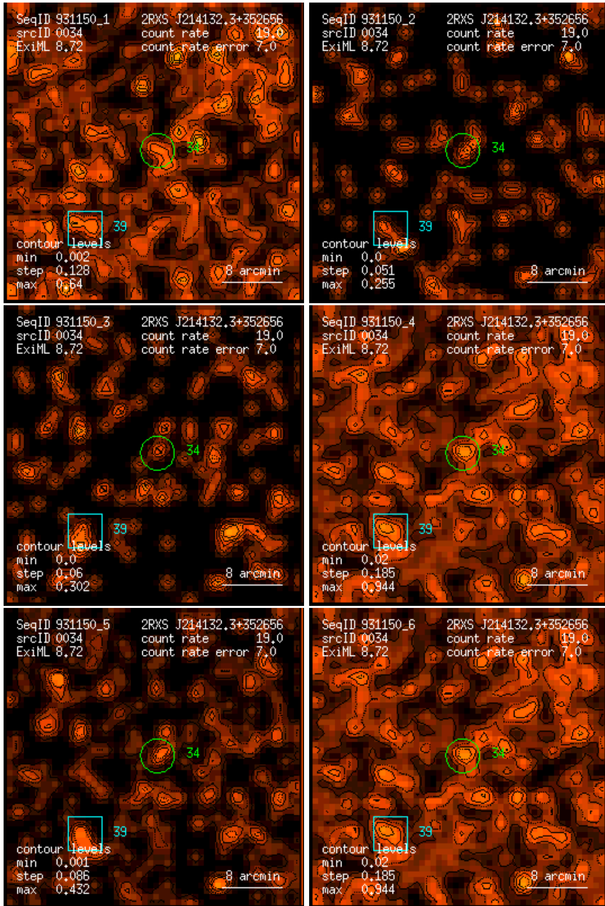
Figure 34: RASS 931150: detection 0034: band rate images, Gaussian filter: (1) PSPC channels 11 – 41, (2) 52 – 90, (3) 91 – 201, (4) 11 – 235, (5) 52 – 201, (6) 11 – 201. Broad band rates in counts/ks. Band rate contour levels in counts/ks/arcmin 2 .
