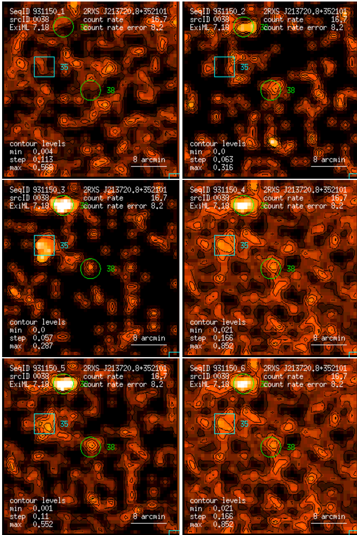
Figure 38: RASS 931150: detection 0038: band rate images, Gaussian filter: (1) PSPC channels 11 – 41, (2) 52 – 90, (3) 91 – 201, (4) 11 – 235, (5) 52 – 201, (6) 11 – 201. Broad band rates in counts/ks. Band rate contour levels in counts/ks/arcmin 2 .
