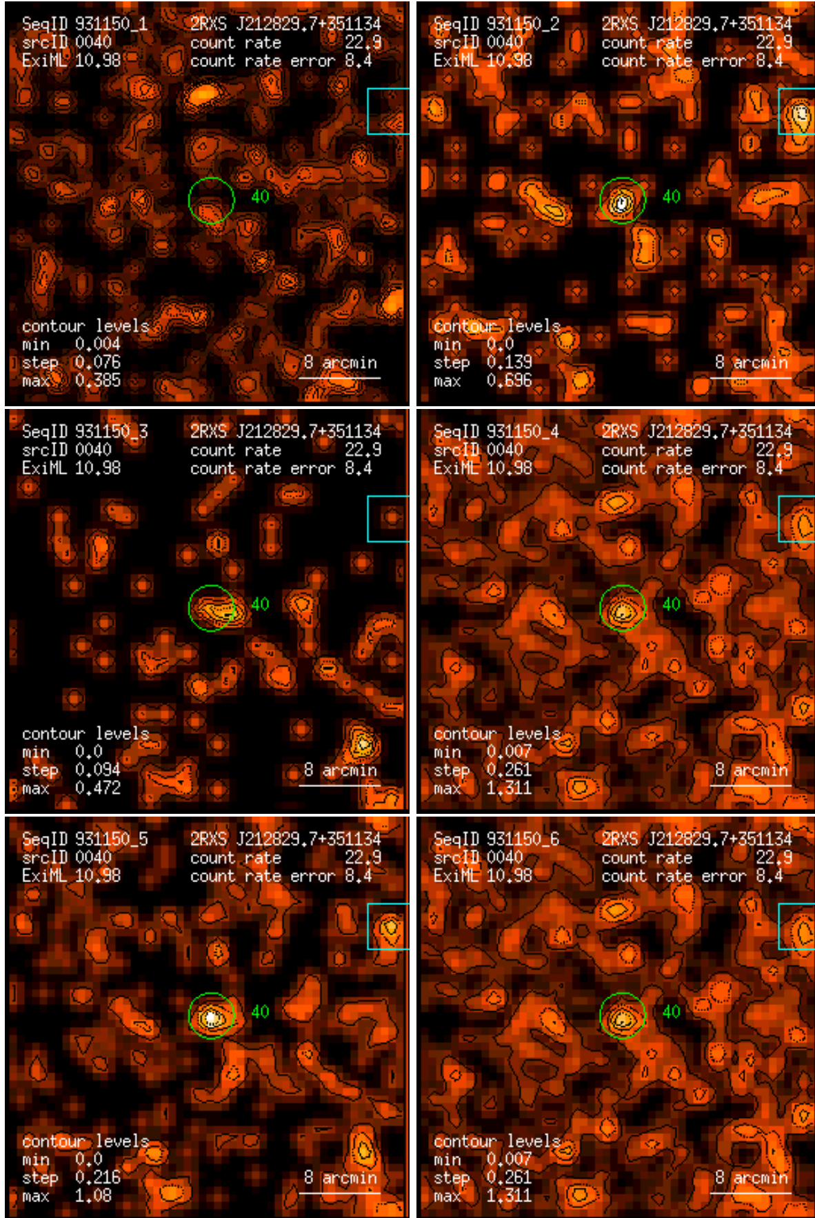
Figure 40: RASS 931150: detection 0040: band rate images, Gaussian filter: (1) PSPC channels 11 – 41, (2) 52 – 90, (3) 91 – 201, (4) 11 – 235, (5) 52 – 201, (6) 11 – 201. Broad band rates in counts/ks. Band rate contour levels in counts/ks/arcmin 2 .
