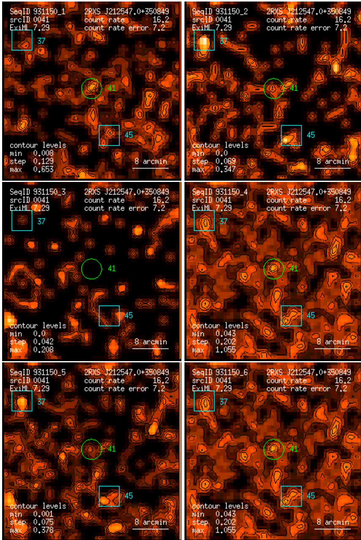
Figure 41: RASS 931150: detection 0041: band rate images, Gaussian filter: (1) PSPC channels 11 – 41, (2) 52 – 90, (3) 91 – 201, (4) 11 – 235, (5) 52 – 201, (6) 11 – 201. Broad band rates in counts/ks. Band rate contour levels in counts/ks/arcmin 2 .
