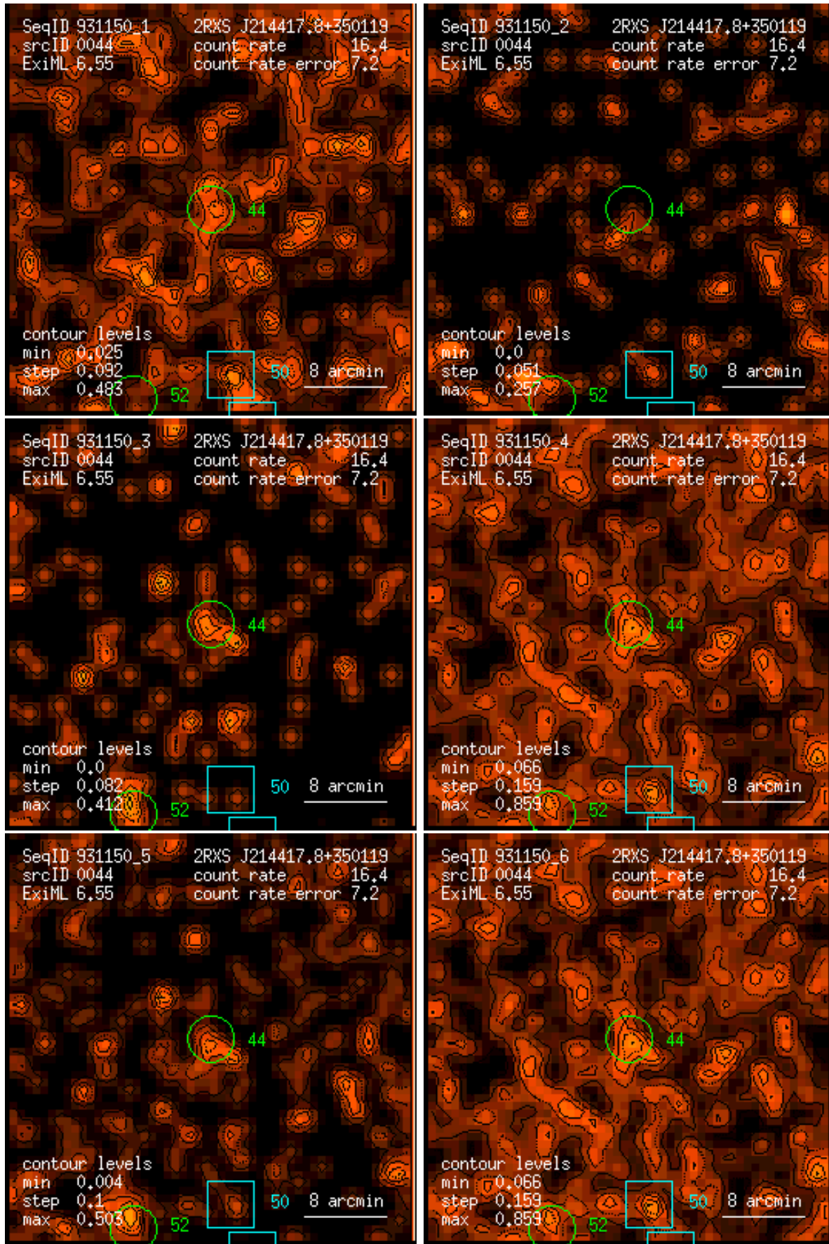
Figure 44: RASS 931150: detection 0044: band rate images, Gaussian filter: (1) PSPC channels 11 – 41, (2) 52 – 90, (3) 91 – 201, (4) 11 – 235, (5) 52 – 201, (6) 11 – 201. Broad band rates in counts/ks. Band rate contour levels in counts/ks/arcmin 2 .
