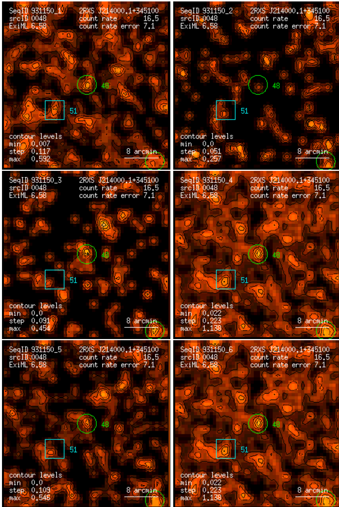
Figure 48: RASS 931150: detection 0048: band rate images, Gaussian filter: (1) PSPC channels 11 – 41, (2) 52 – 90, (3) 91 – 201, (4) 11 – 235, (5) 52 – 201, (6) 11 – 201. Broad band rates in counts/ks. Band rate contour levels in counts/ks/arcmin 2 .
