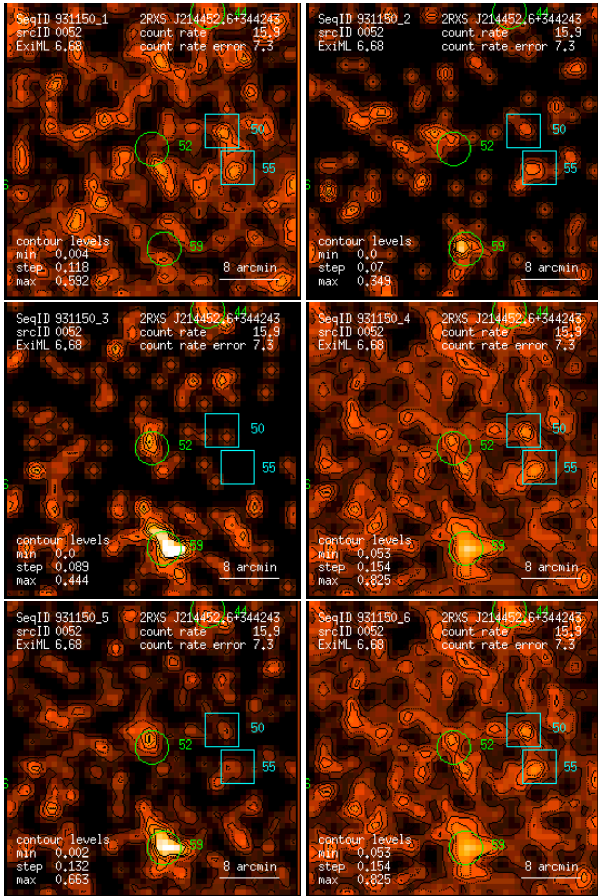
Figure 52: RASS 931150: detection 0052: band rate images, Gaussian filter: (1) PSPC channels 11 – 41, (2) 52 – 90, (3) 91 – 201, (4) 11 – 235, (5) 52 – 201, (6) 11 – 201. Broad band rates in counts/ks. Band rate contour levels in counts/ks/arcmin 2 .
