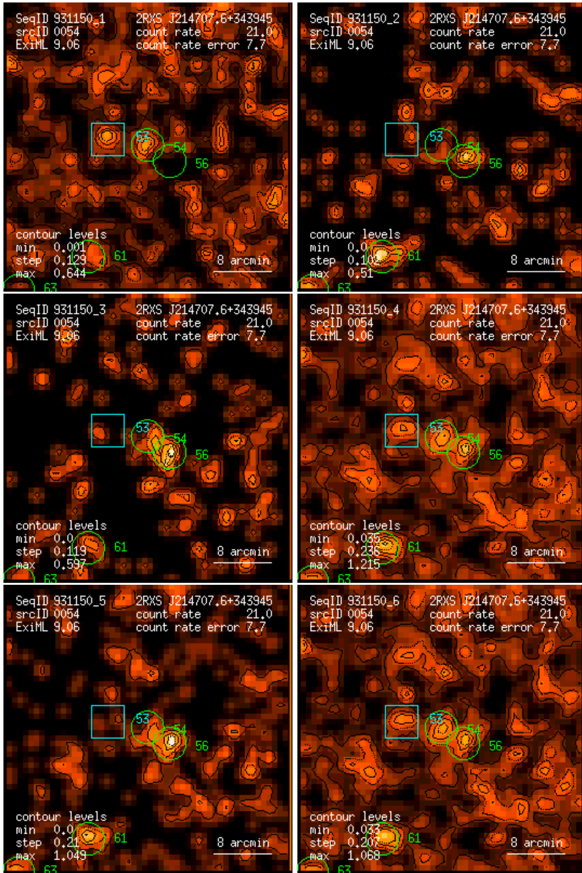
Figure 54: RASS 931150: detection 0054: band rate images, Gaussian filter: (1) PSPC channels 11 – 41, (2) 52 – 90, (3) 91 – 201, (4) 11 – 235, (5) 52 – 201, (6) 11 – 201. Broad band rates in counts/ks. Band rate contour levels in counts/ks/arcmin 2 .
