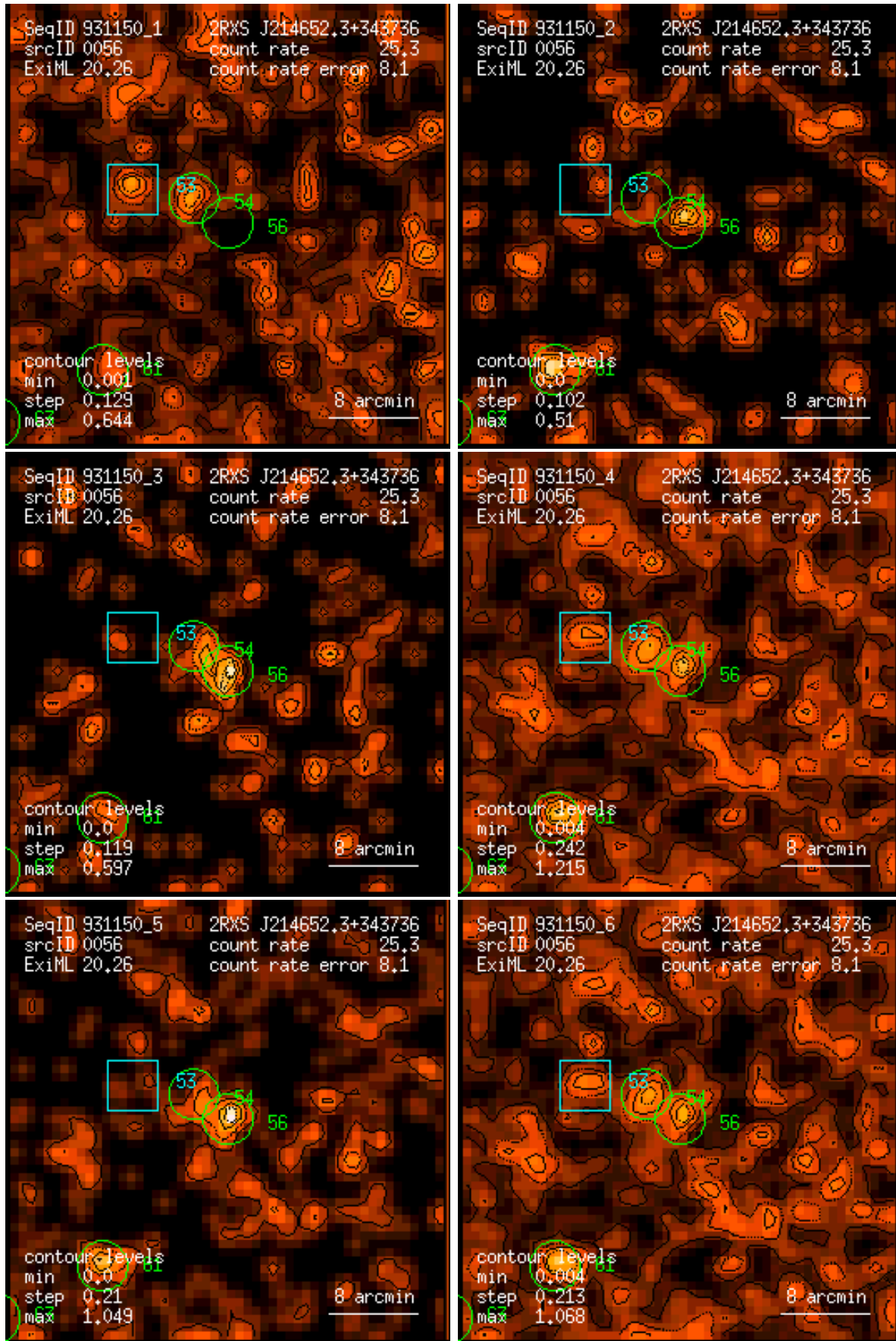
Figure 56: RASS 931150: detection 0056: band rate images, Gaussian filter: (1) PSPC channels 11 – 41, (2) 52 – 90, (3) 91 – 201, (4) 11 – 235, (5) 52 – 201, (6) 11 – 201. Broad band rates in counts/ks. Band rate contour levels in counts/ks/arcmin 2 .
