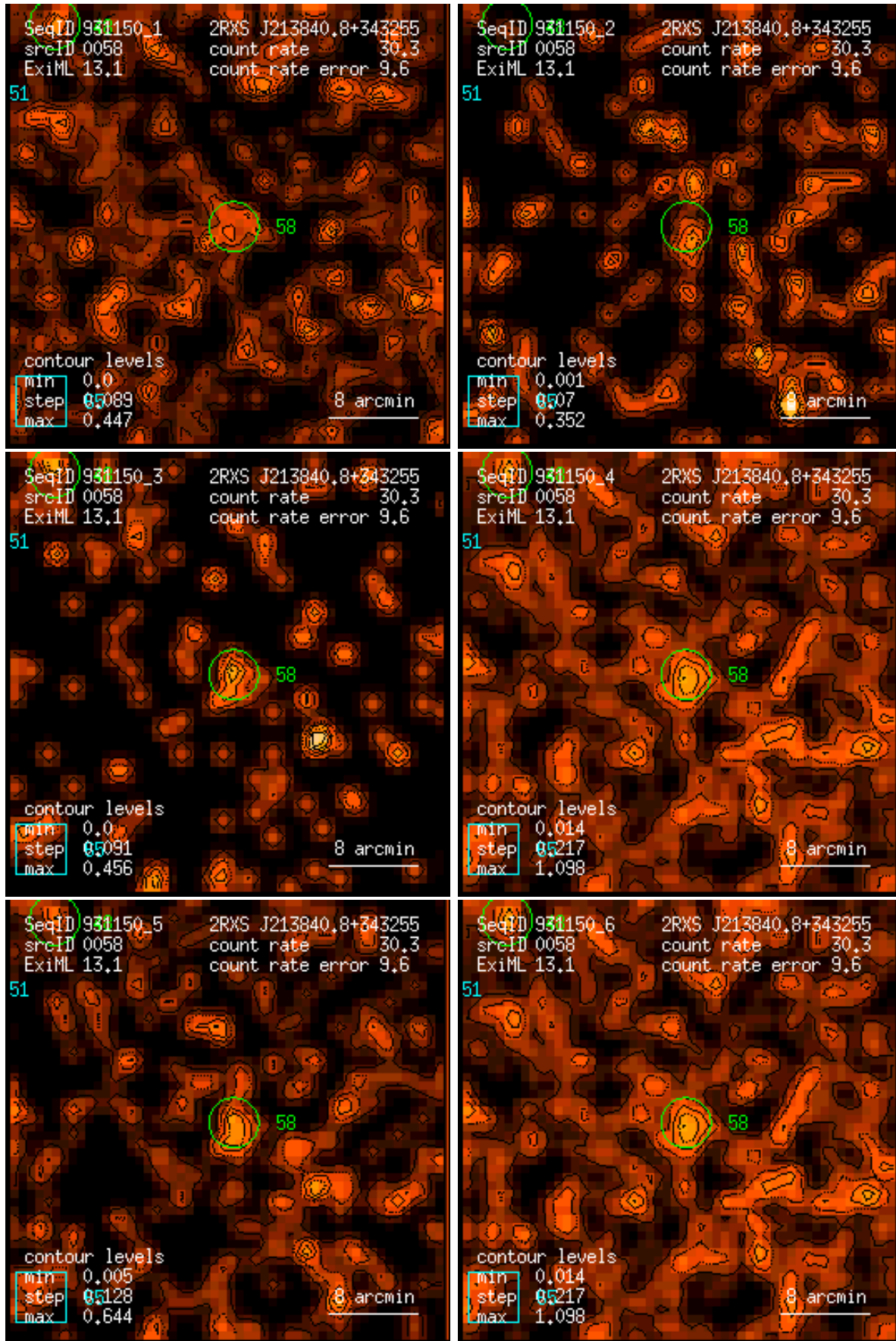
Figure 58: RASS 931150: detection 0058: band rate images, Gaussian filter: (1) PSPC channels 11 – 41, (2) 52 – 90, (3) 91 – 201, (4) 11 – 235, (5) 52 – 201, (6) 11 – 201. Broad band rates in counts/ks. Band rate contour levels in counts/ks/arcmin 2 .
