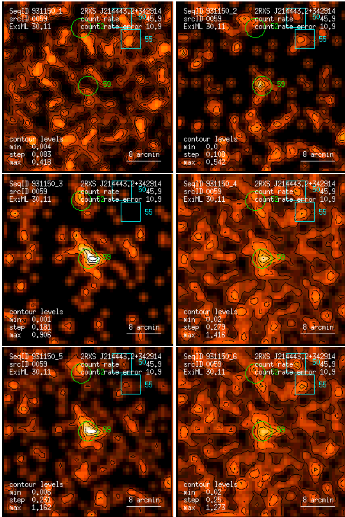
Figure 59: RASS 931150: detection 0059: band rate images, Gaussian filter: (1) PSPC channels 11 – 41, (2) 52 – 90, (3) 91 – 201, (4) 11 – 235, (5) 52 – 201, (6) 11 – 201. Broad band rates in counts/ks. Band rate contour levels in counts/ks/arcmin 2 .
