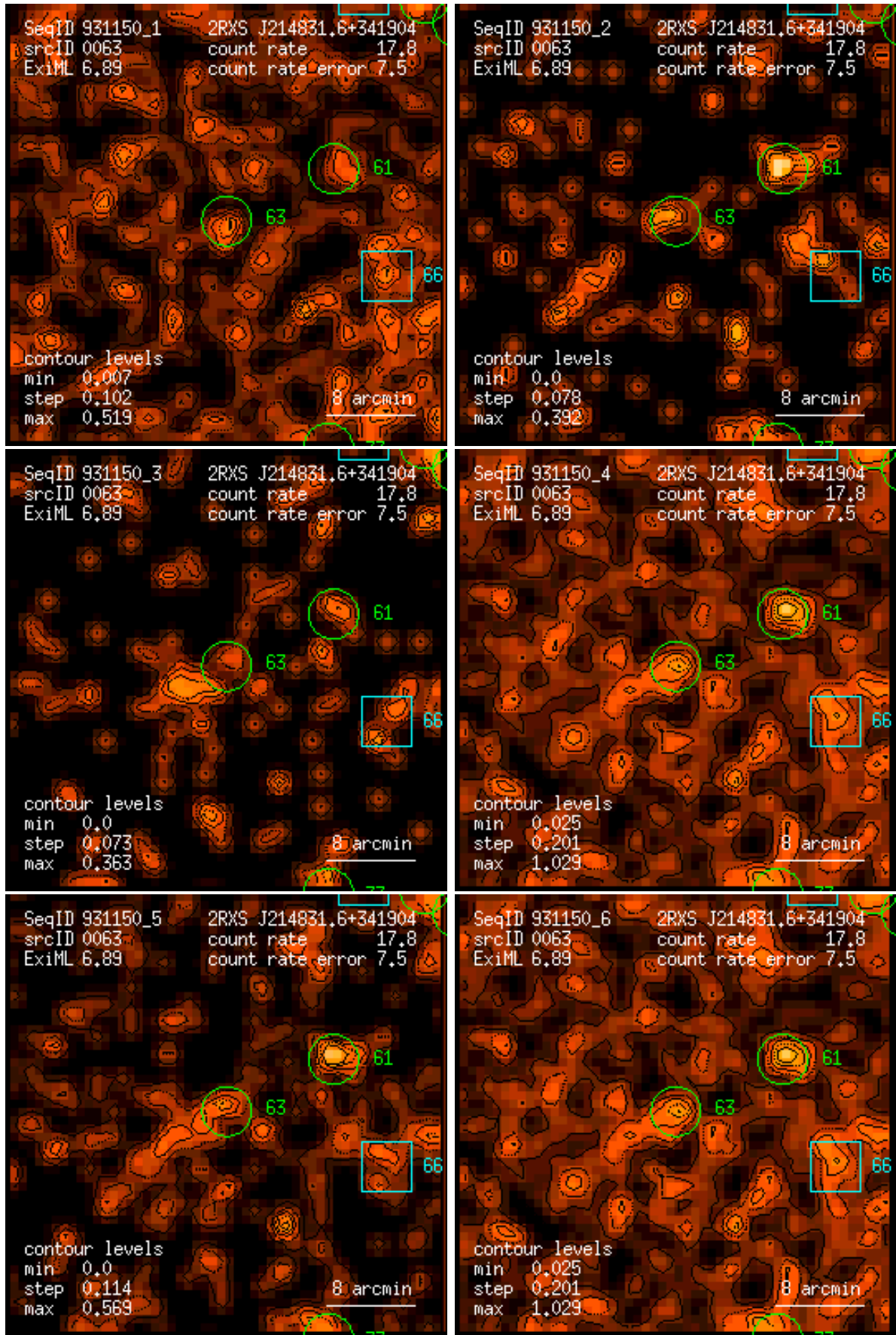
Figure 63: RASS 931150: detection 0063: band rate images, Gaussian filter: (1) PSPC channels 11 – 41, (2) 52 – 90, (3) 91 – 201, (4) 11 – 235, (5) 52 – 201, (6) 11 – 201. Broad band rates in counts/ks. Band rate contour levels in counts/ks/arcmin 2 .
